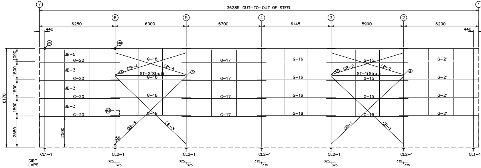
SIDEWALL FRAMING: FRAME LINE C
