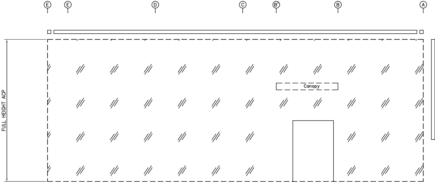
SIDEWALL SHEETING & TRIM: FRAME LINE 5
