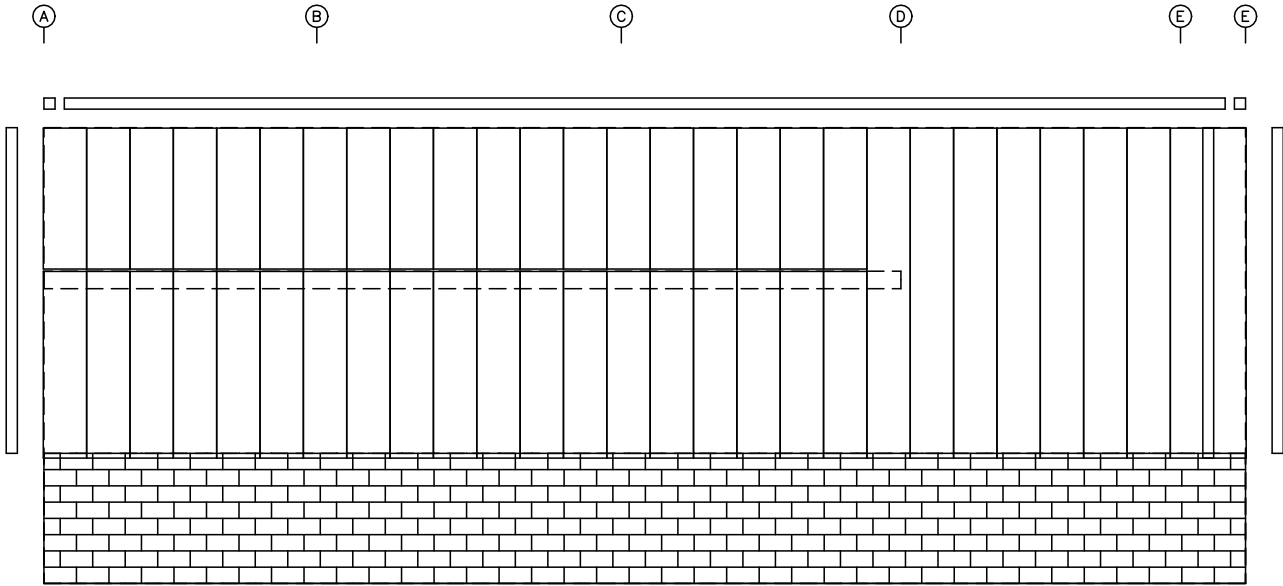
SIDEWALL SHEETING & TRIM: FRAME LINE 1
