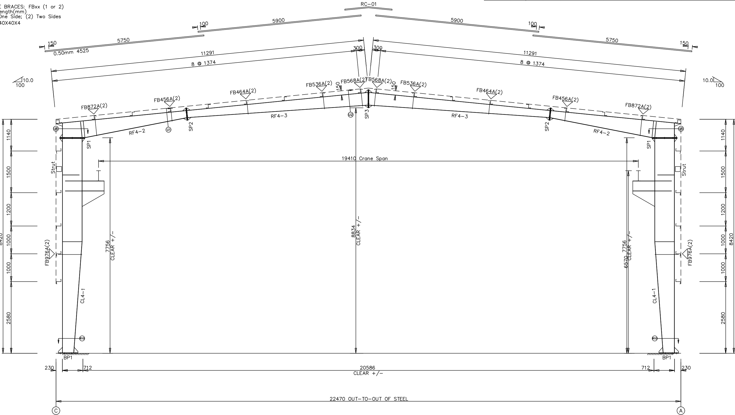
RIGID FRAME ELEVATION: FRAME LINE 6
