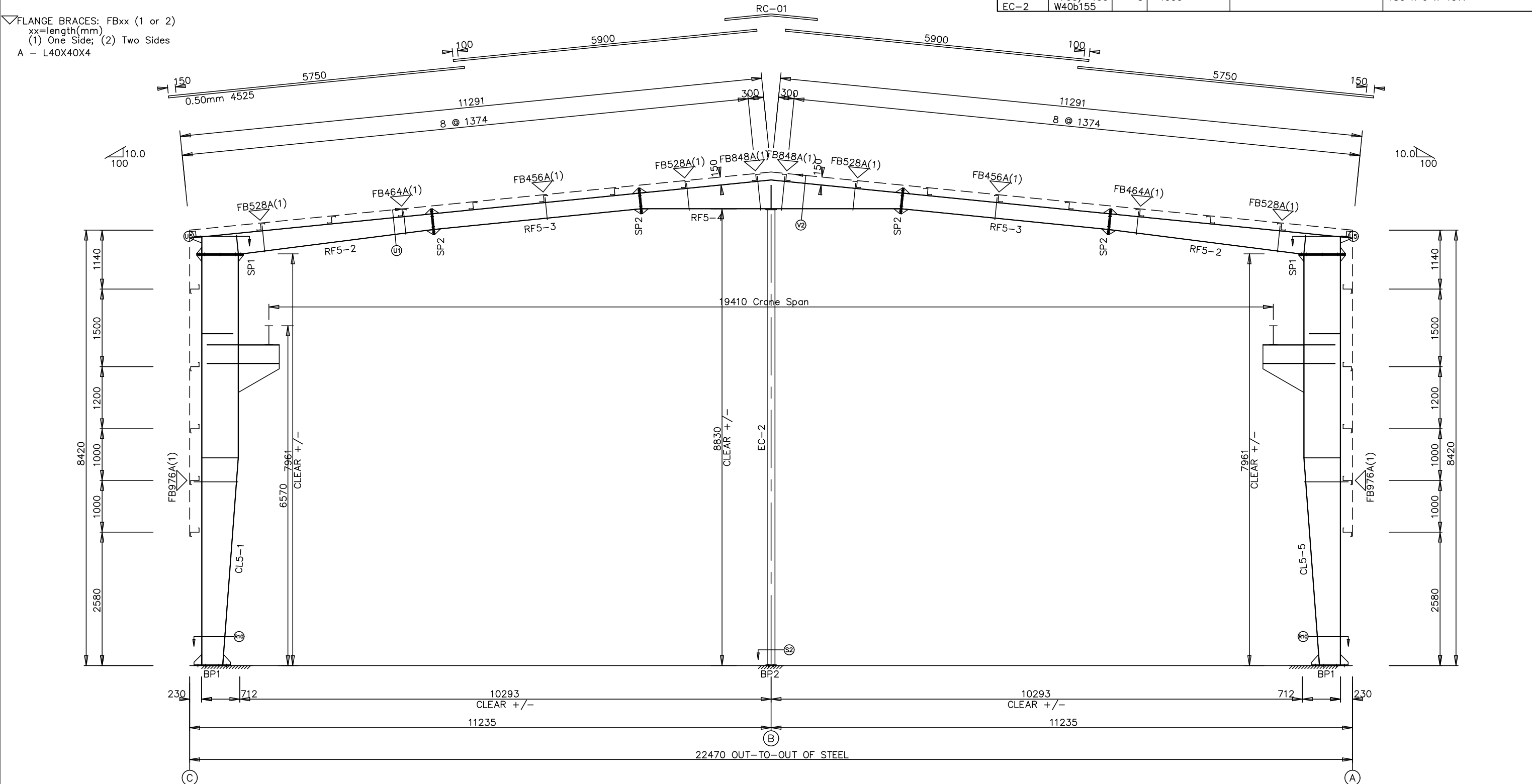
RIGID FRAME ELEVATION: FRAME LINE 7
