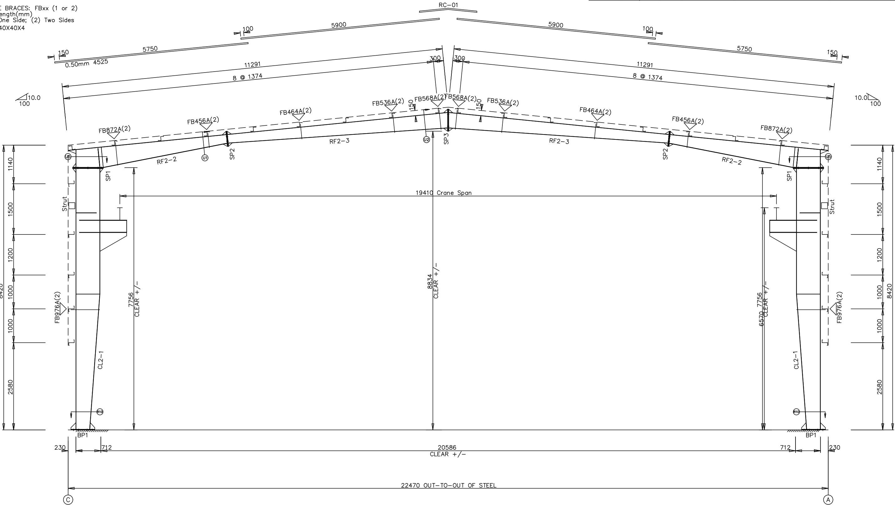
RIGID FRAME ELEVATION: FRAME LINE 2 3 5
