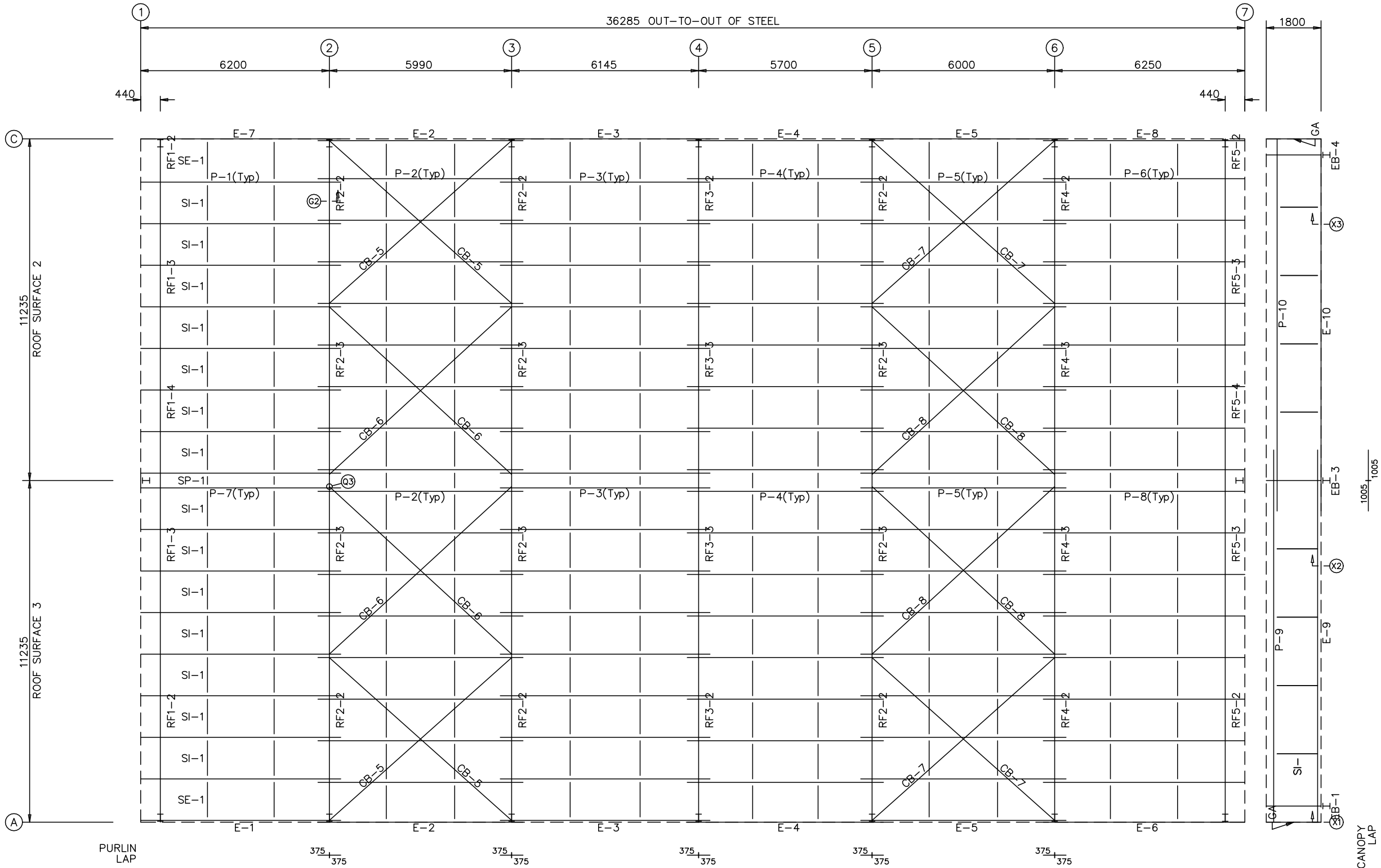
COLUMNS & RAFTERS MARKING PLAN
