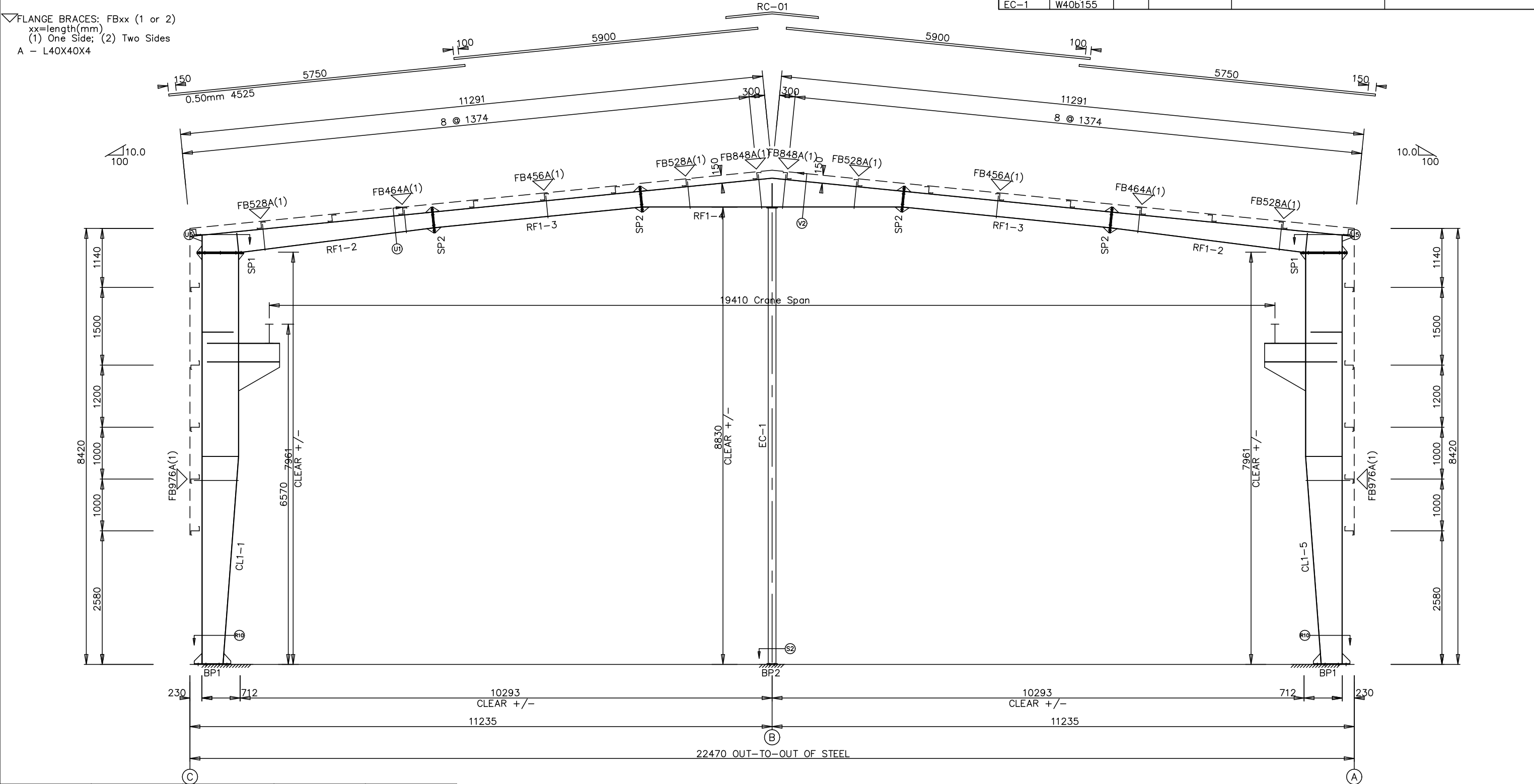
RIGID FRAME ELEVATION: FRAME LINE 1
