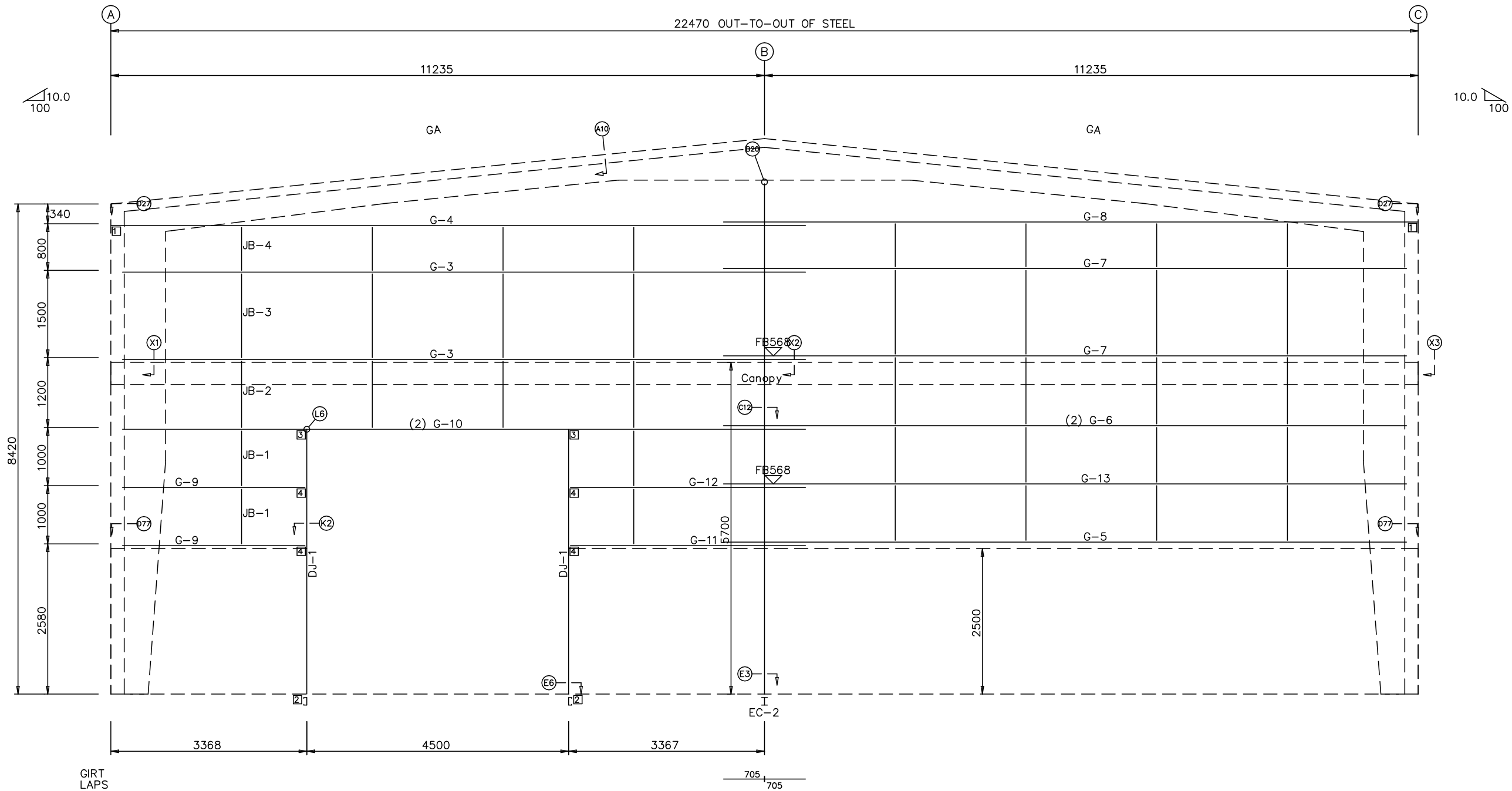
ENDWALL FRAMING: FRAME LINE 7
