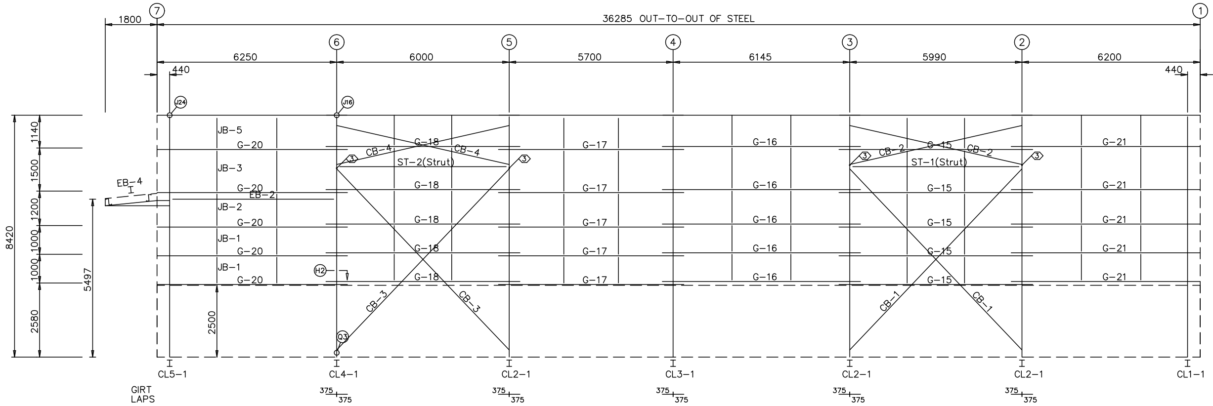
SIDEWALL FRAMING: FRAME LINE C
