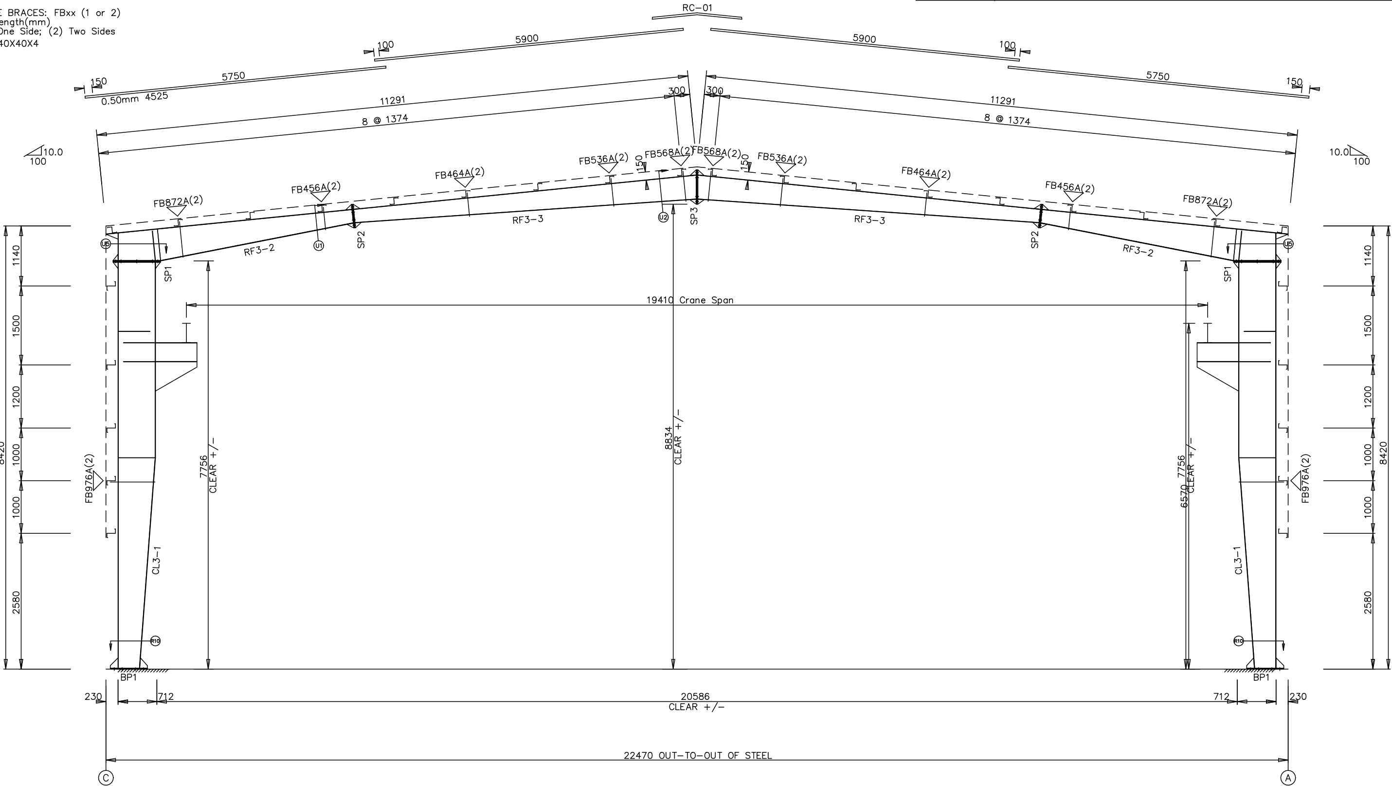
RIGID FRAME ELEVATION: FRAME LINE 4
