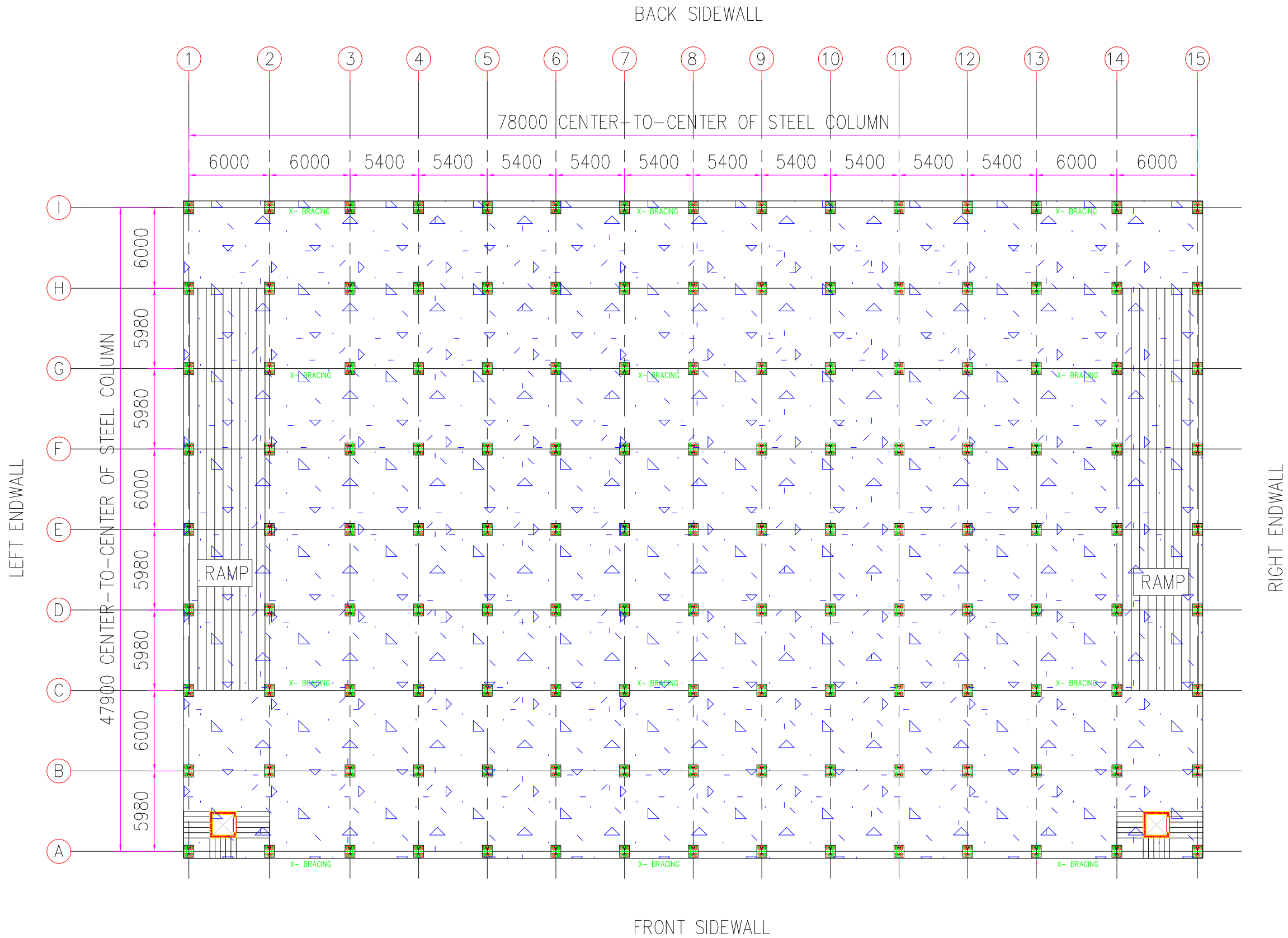
FLOOR PLAN @ LVL.+3.1m, 6.2m, 9.3m, 12.4m, 15.5m, 18.6m, 21.7m, 24.8m, 27.9m, 31.0m
