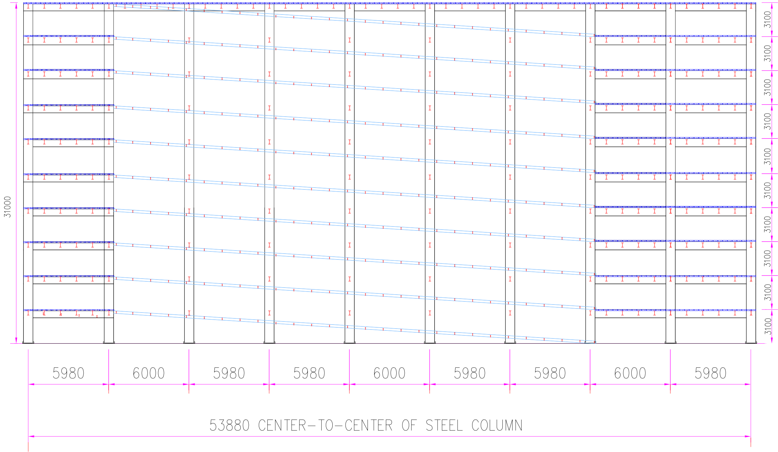
SECTION X-X
