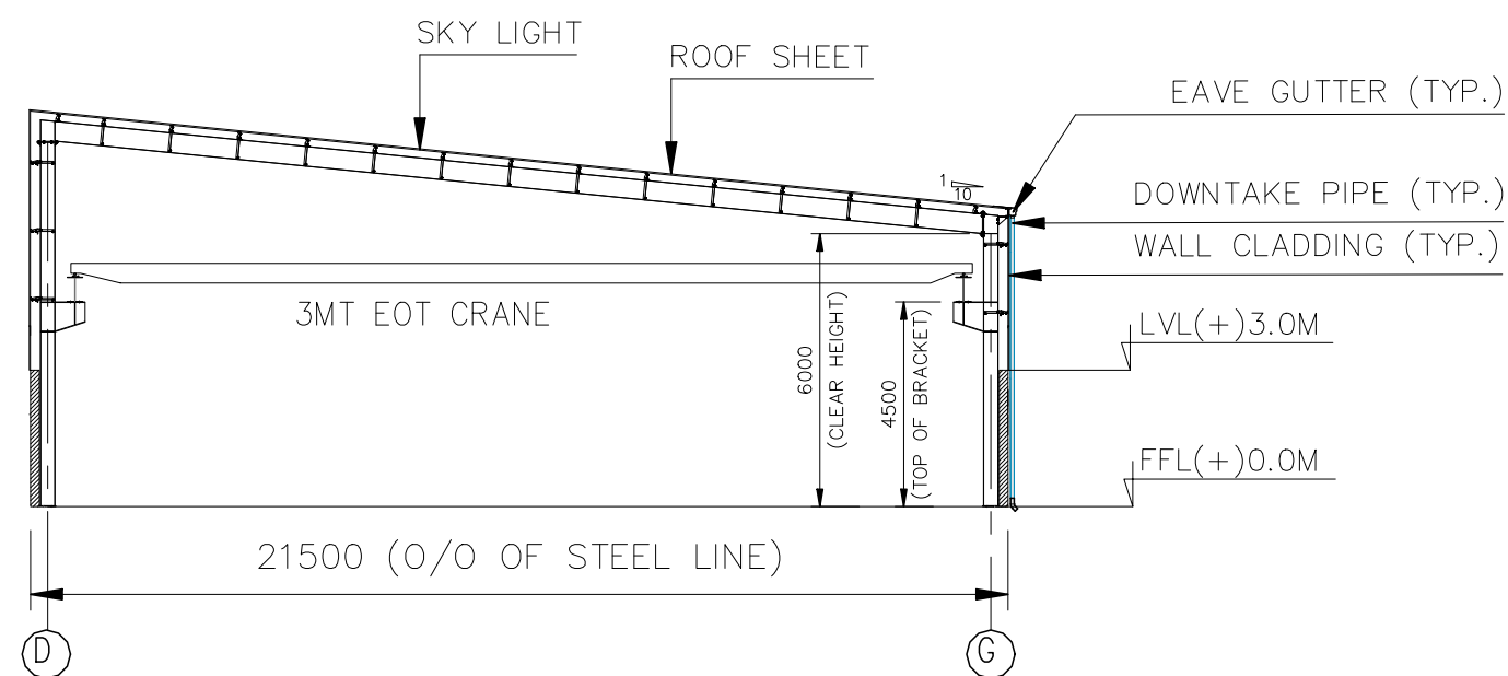
TYPICAL FRAME ELEVATION
