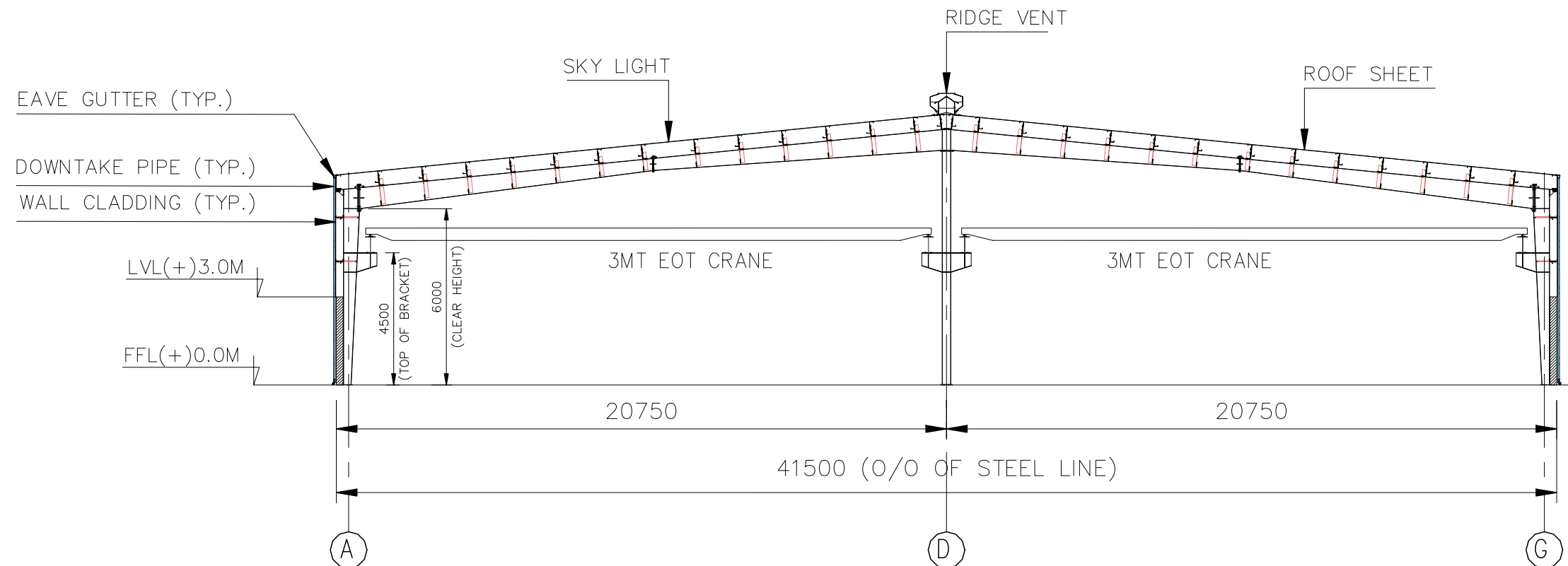
TYPICAL FRAME ELEVATION
