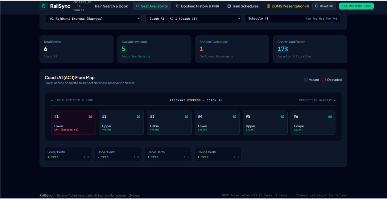
Figure 5: Seat availability and coach floor map.
