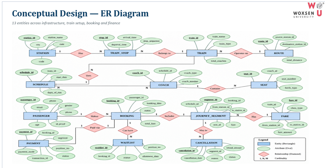
Figure 1: Entity-Relationship diagram for the railway reservation database.
