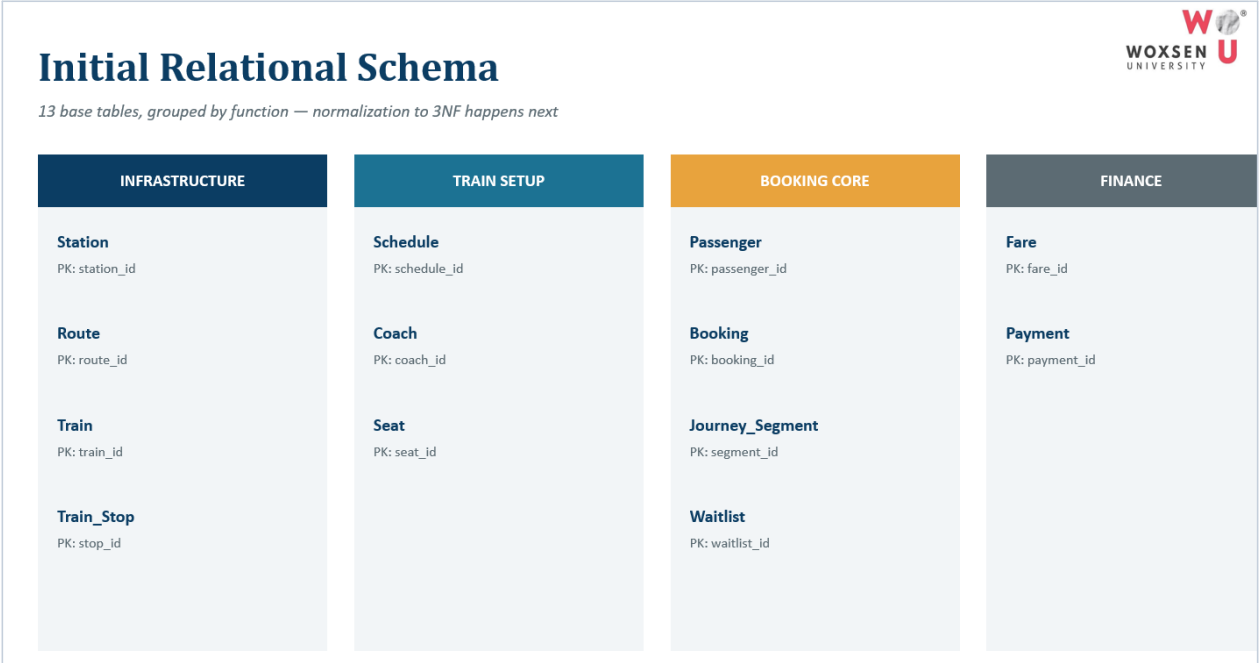
Figure 2: Relational schema supplied for the project.
