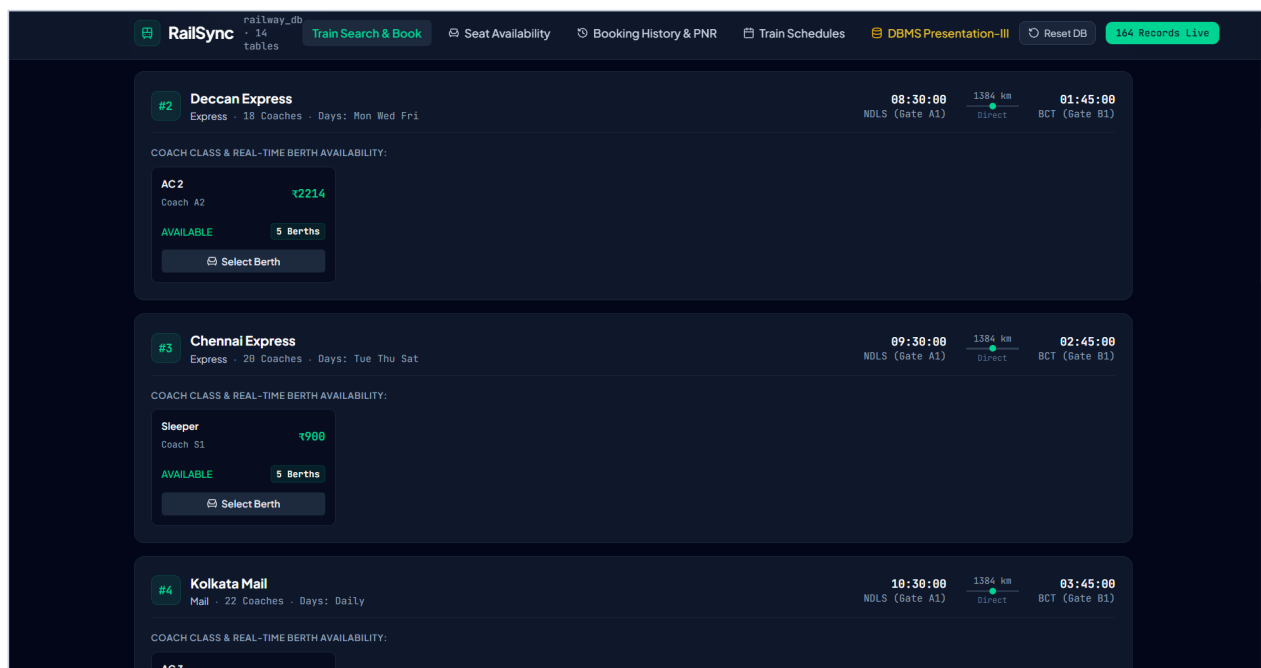
Figure 4: Train search results with class-wise berth availability.
