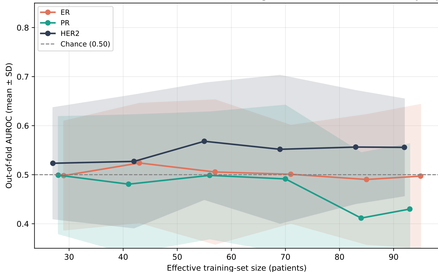
Learning curves — AUROC vs training-set size (elastic-net, radiomic block of 642 features, leakage-safe nested folds; 25 folds per point)
