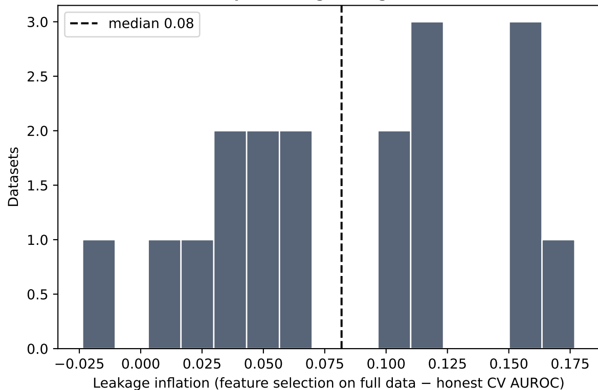
B. Preprocessing-leakage inflation
