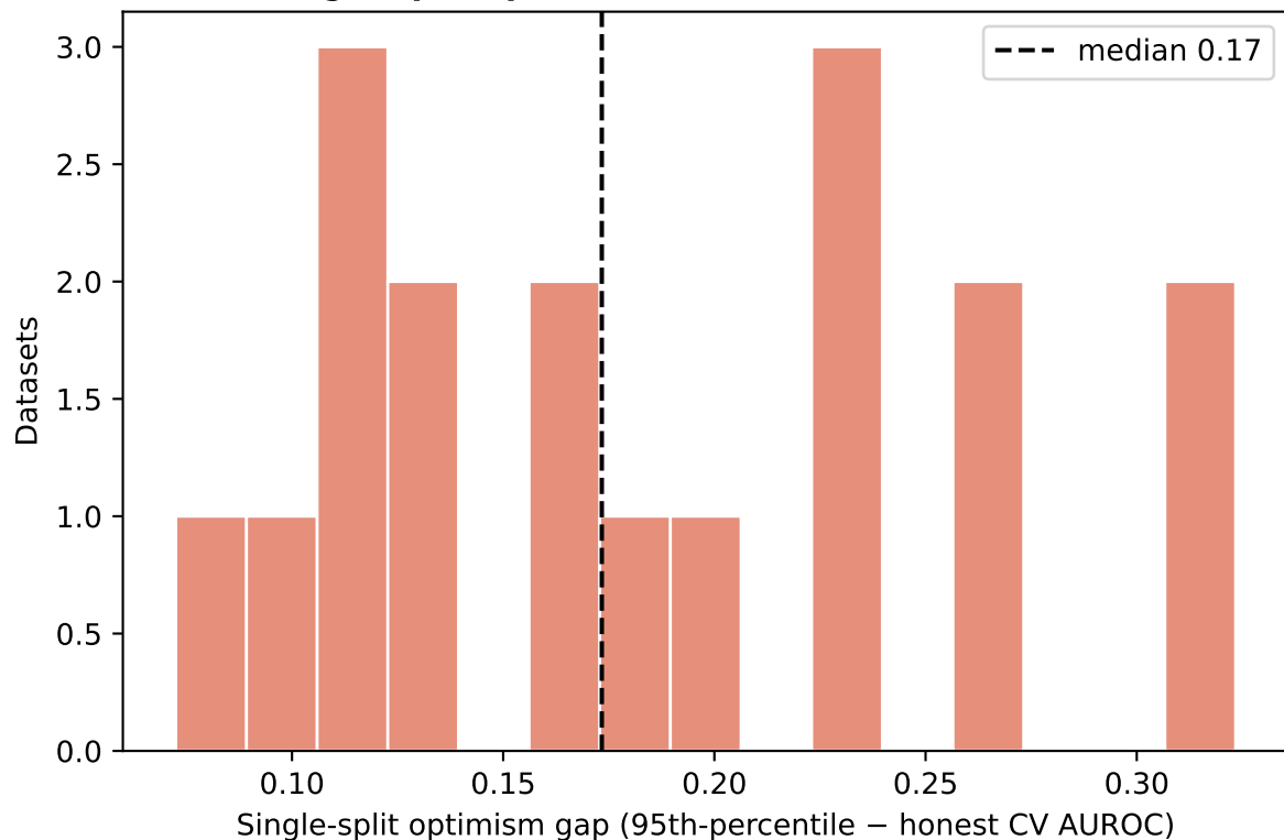
A. Single-split optimism across 18 radiomics datasets
