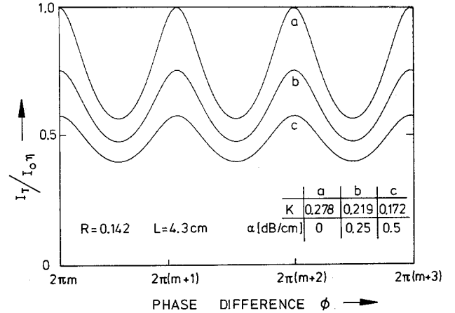
Fig. 2. Calculated resonator transmission versus phase difference. Parameters are resonator length L , end-face reflectivity R and attenuation coefficients \alpha (see inset). K is the corresponding contrast
