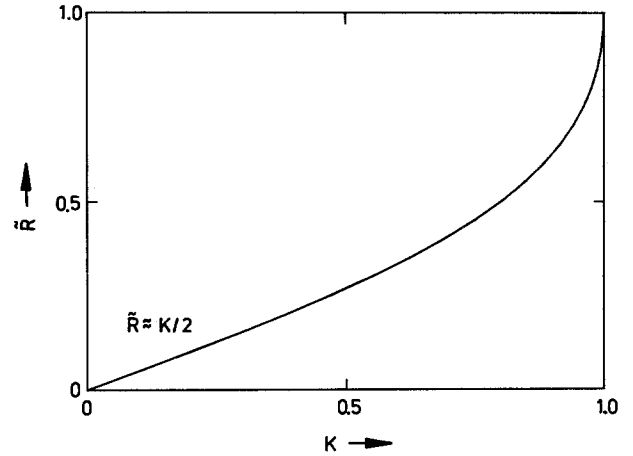
Fig. 3. Combined loss-reflection factor \tilde{R} = R \exp(-\alpha L) as function of the resonances' contrast K
