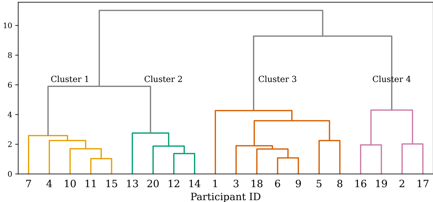
Ward linkage height
