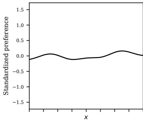
Overall Mean
