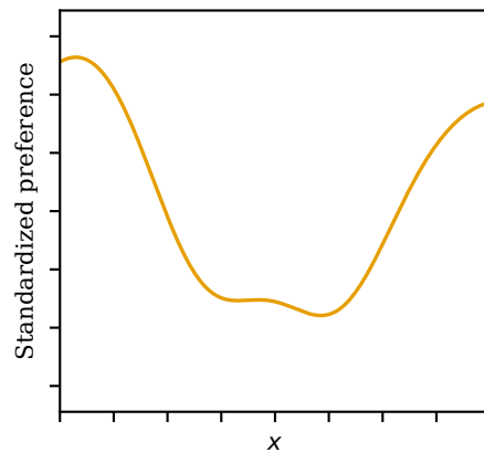
Cluster 1 Mean
