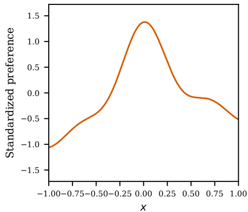
Cluster 3 Mean
