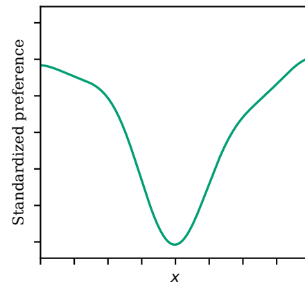
Cluster 2 Mean
