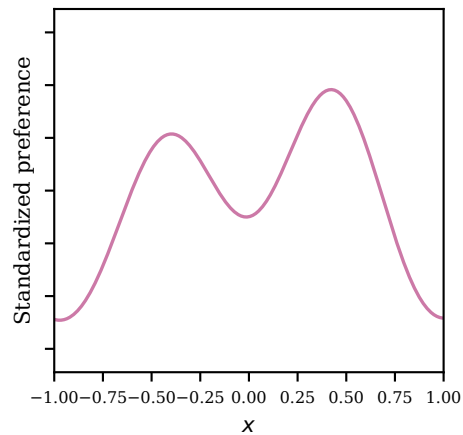
Cluster 4 Mean
