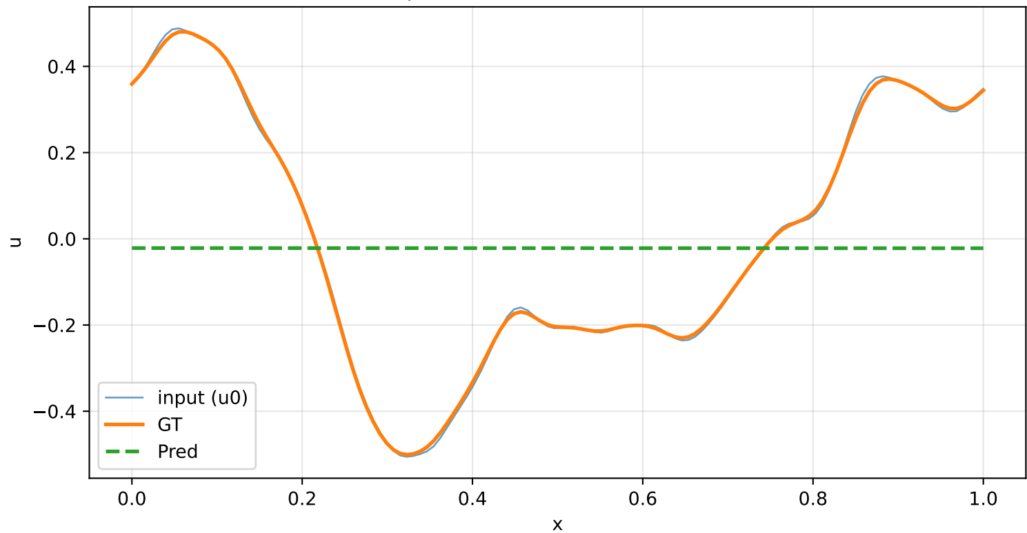
sample 1, t=0: relL2=1 RMSE=0.3
