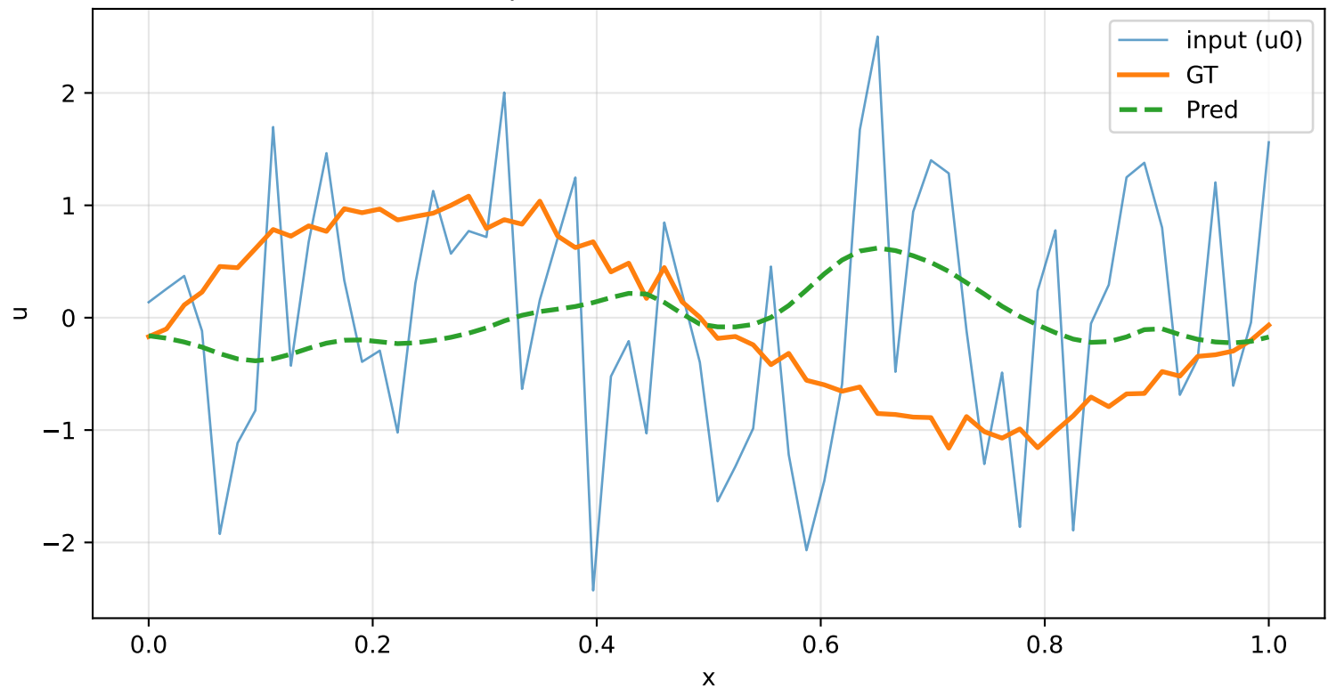
sample 2: relL2=1.21 RMSE=0.858
