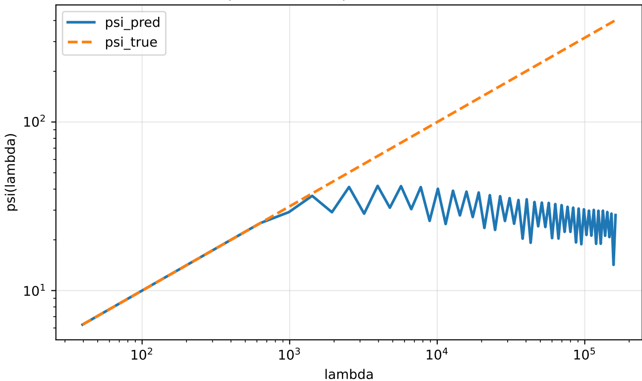
psi baseline (split=all, N=220)
