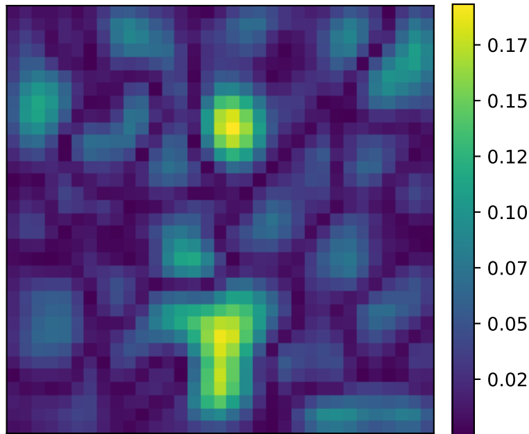
|Pred-GT|
