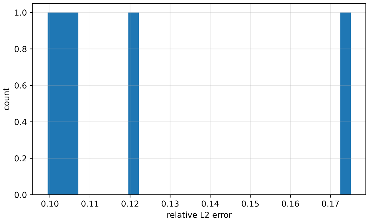
PSRSDNO test relL2 (lambda=0, mean=0.121, median=0.106)
