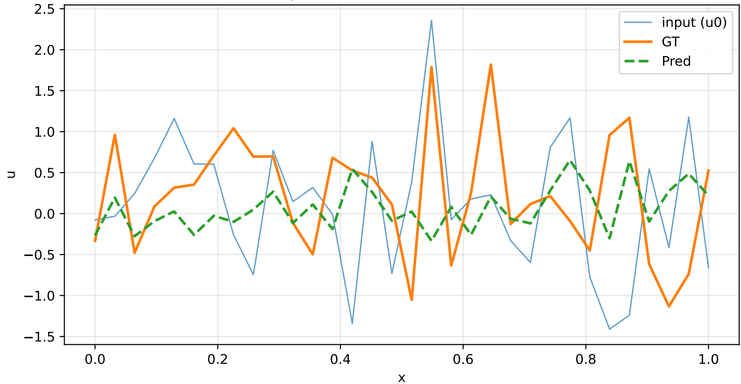
sample 2: relL2=1.06 RMSE=0.803
