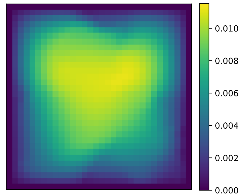
GT
