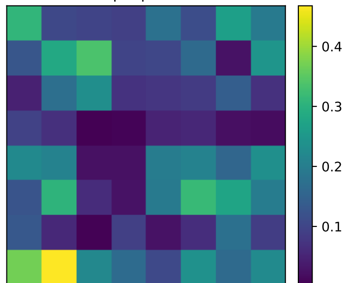
|\text{Err}| t=3
