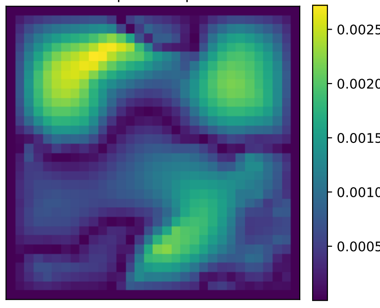
|Pred-GT|
