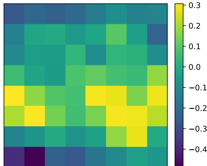
GT t=3
