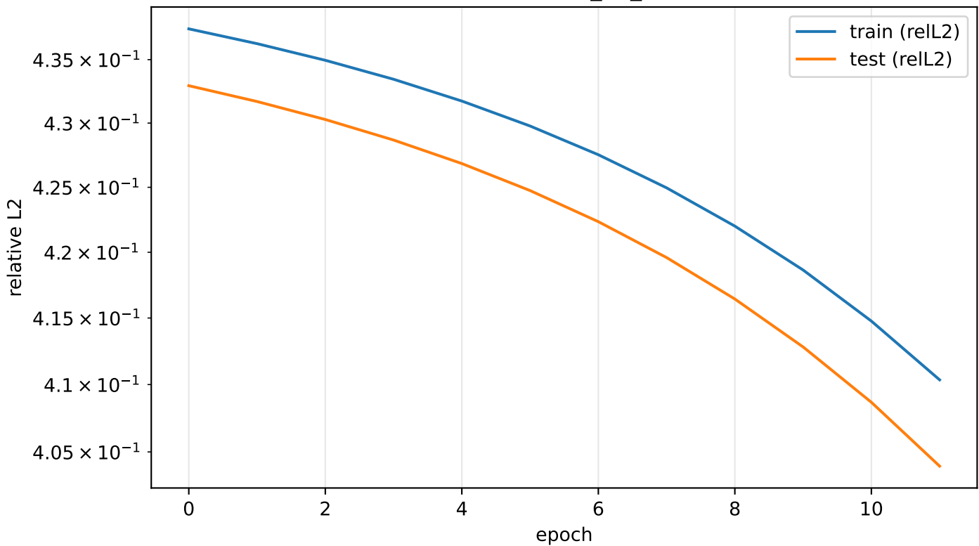
subordination_1d_time
