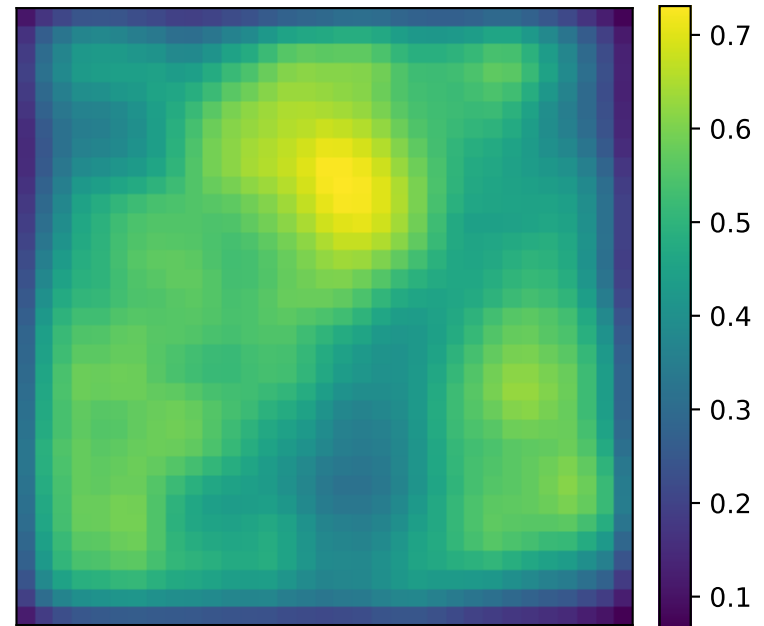
GT
