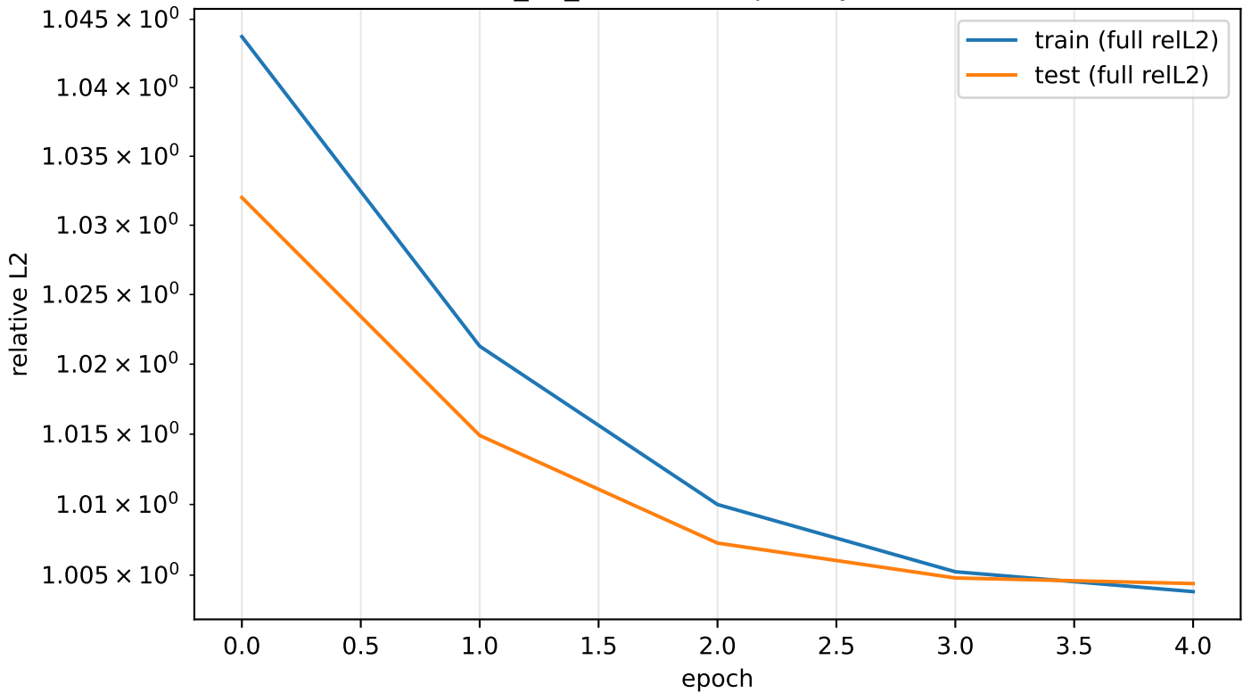
fourier_1d_time: full-trajectory relative L2
