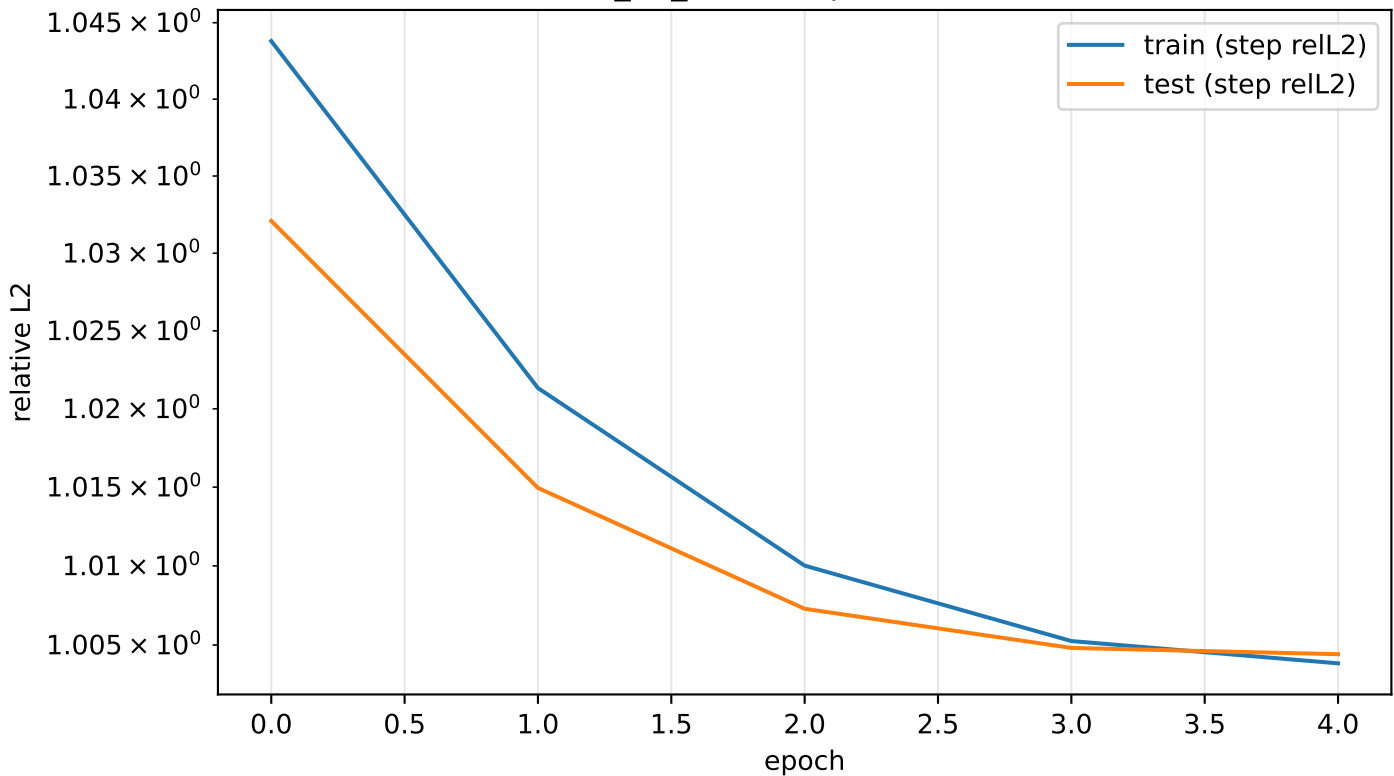
fourier_1d_time: stepwise relative L2
