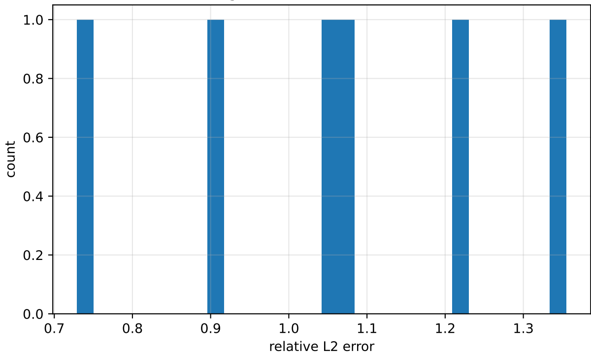
error histogram (mean=1.06, median=1.07)
