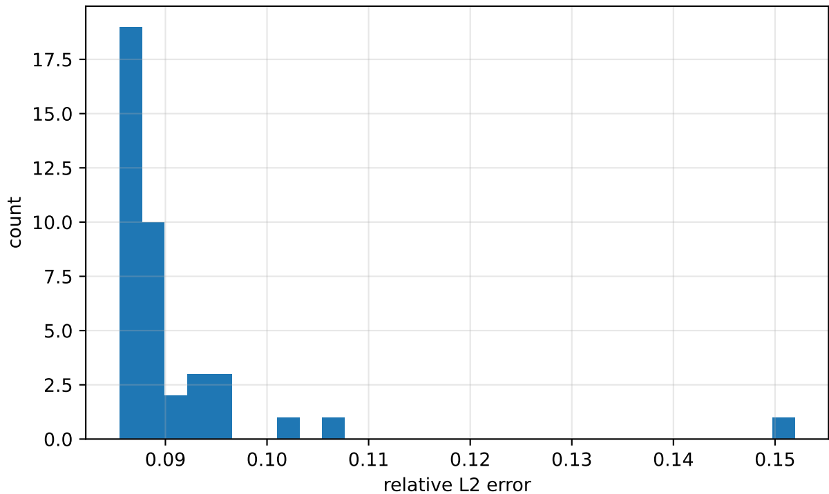
error histogram (mean=0.091, median=0.0879)
