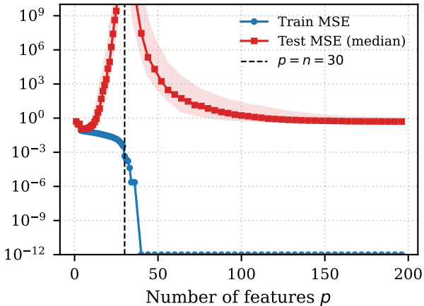
Double descent ( n = 30 , varying p )
