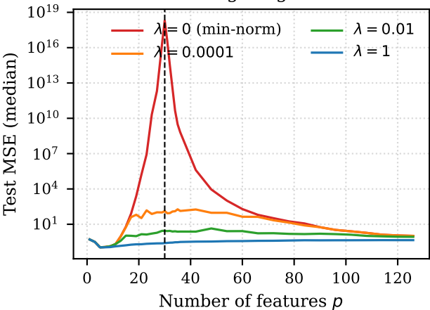
Effect of ridge regularization
