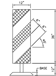
OVERSIZED VERTICAL PANEL
