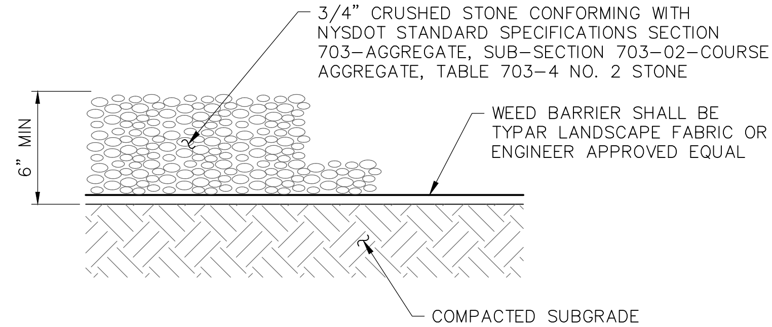
2 GRAVEL SURFACING TREATMENT SCALE: 1/2" = 1'-0" (11x17 SIZE) 1 1/2" = 1'-0" (22x34 SIZE)
