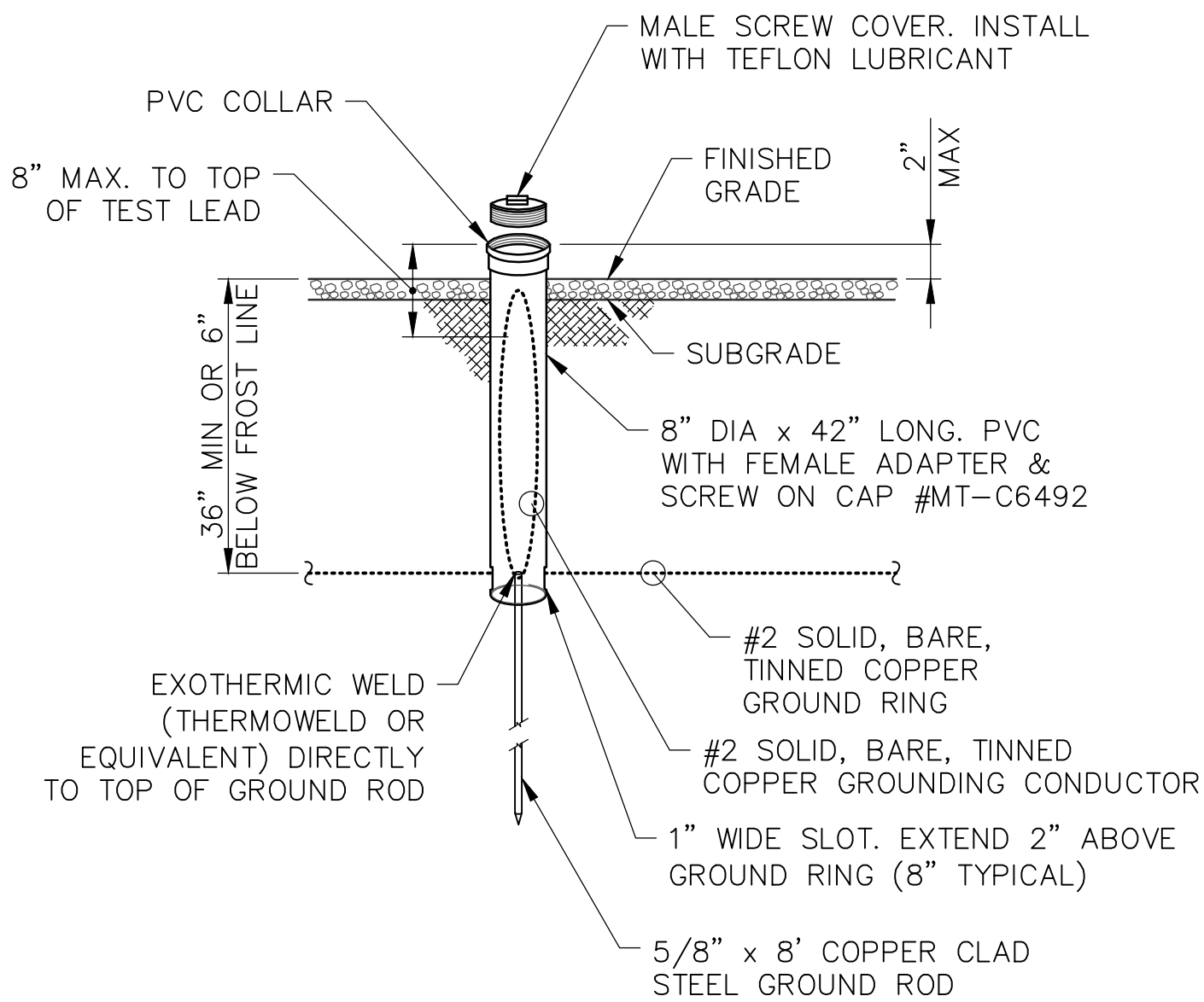
1 GROUND ROD WITH TEST WELL SCALE: NTS
