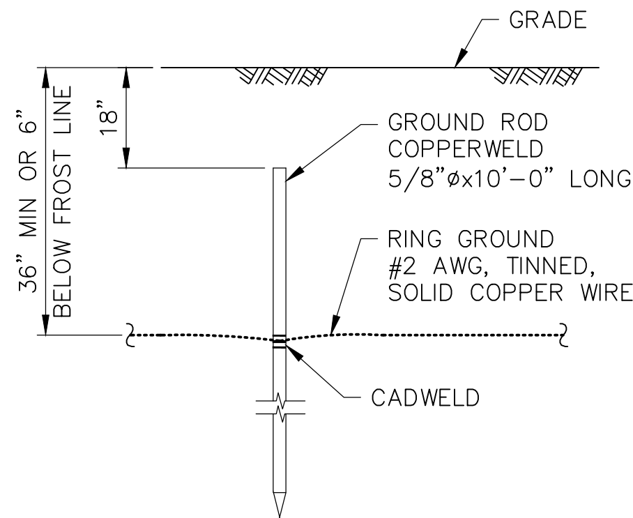
2 GROUND ROD SCALE: NTS
