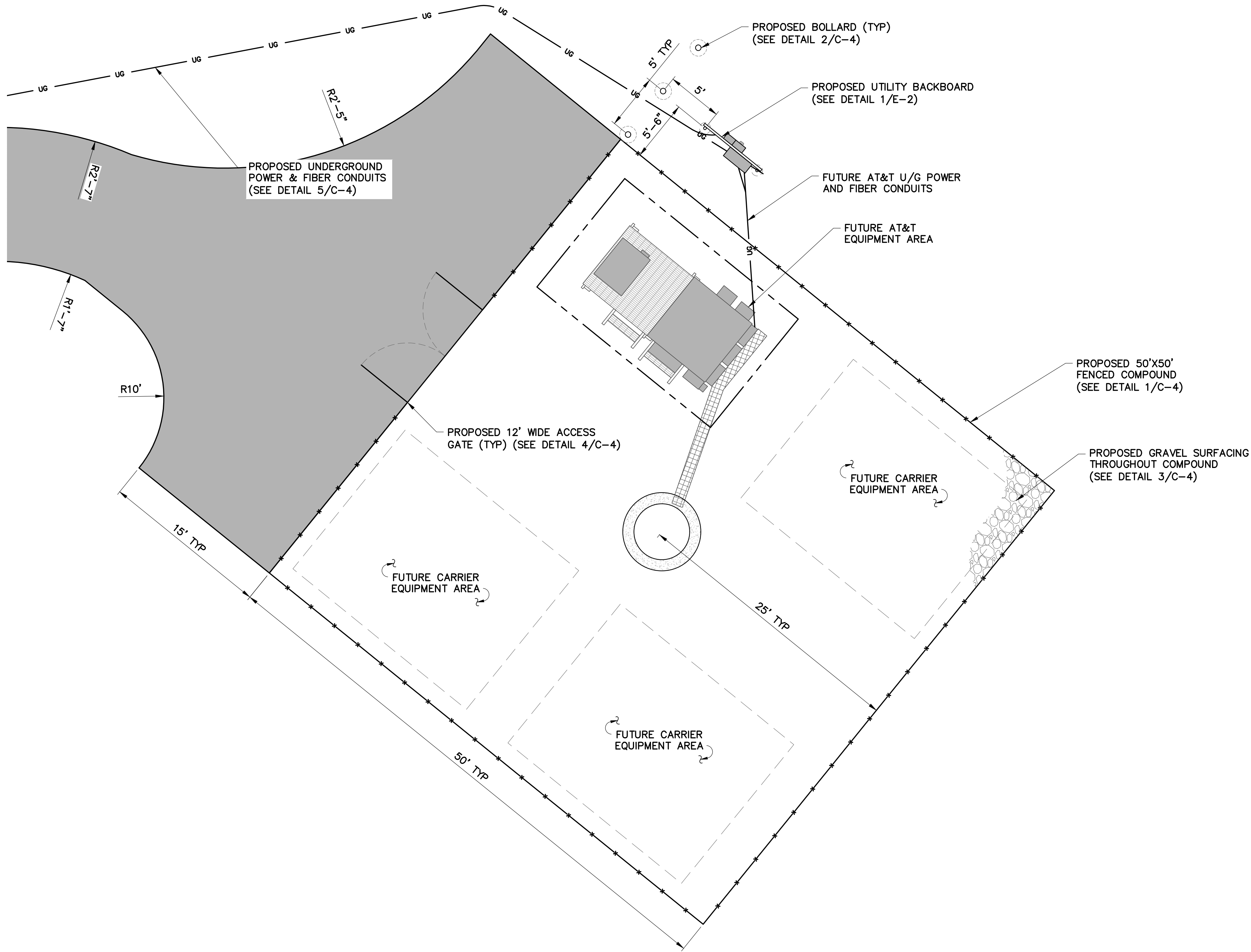
1 C-2 SITE DETAIL PLAN SCALE: 1" = 10' (11x17 SIZE) 1" = 5' (22x34 SIZE)
