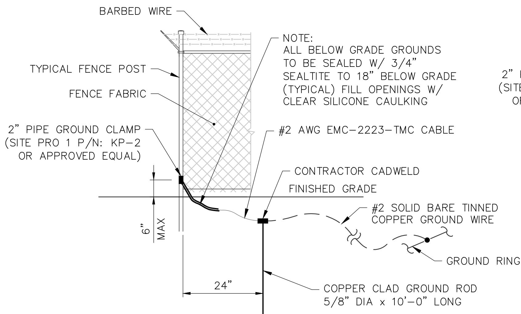
6 FENCE CORNER GROUNDING DETAIL SCALE: NTS
