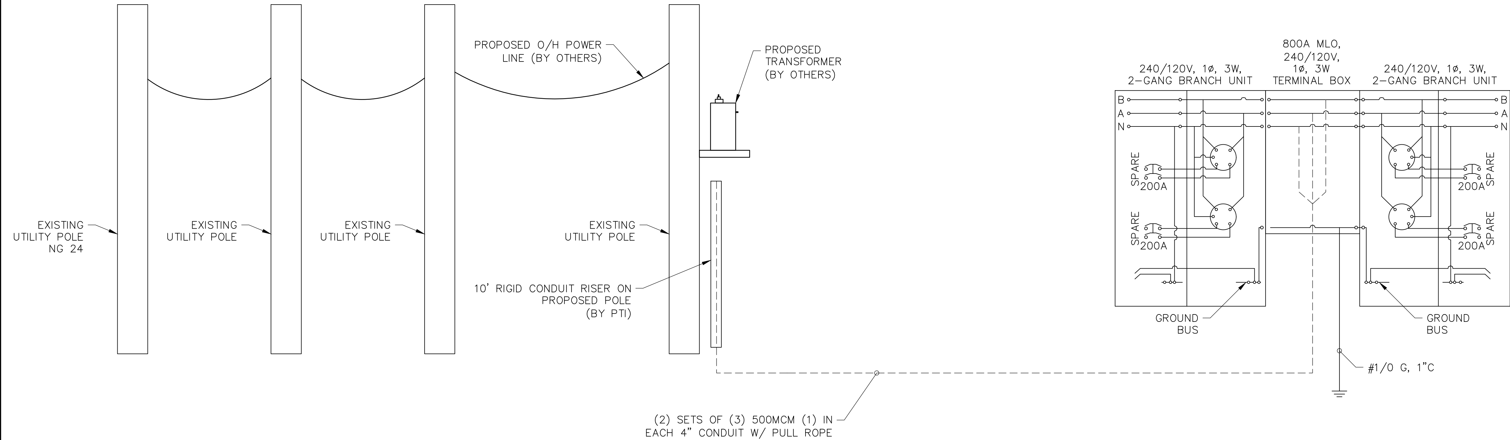
1 SINGLE LINE DIAGRAM E-1 SCALE: NTS
