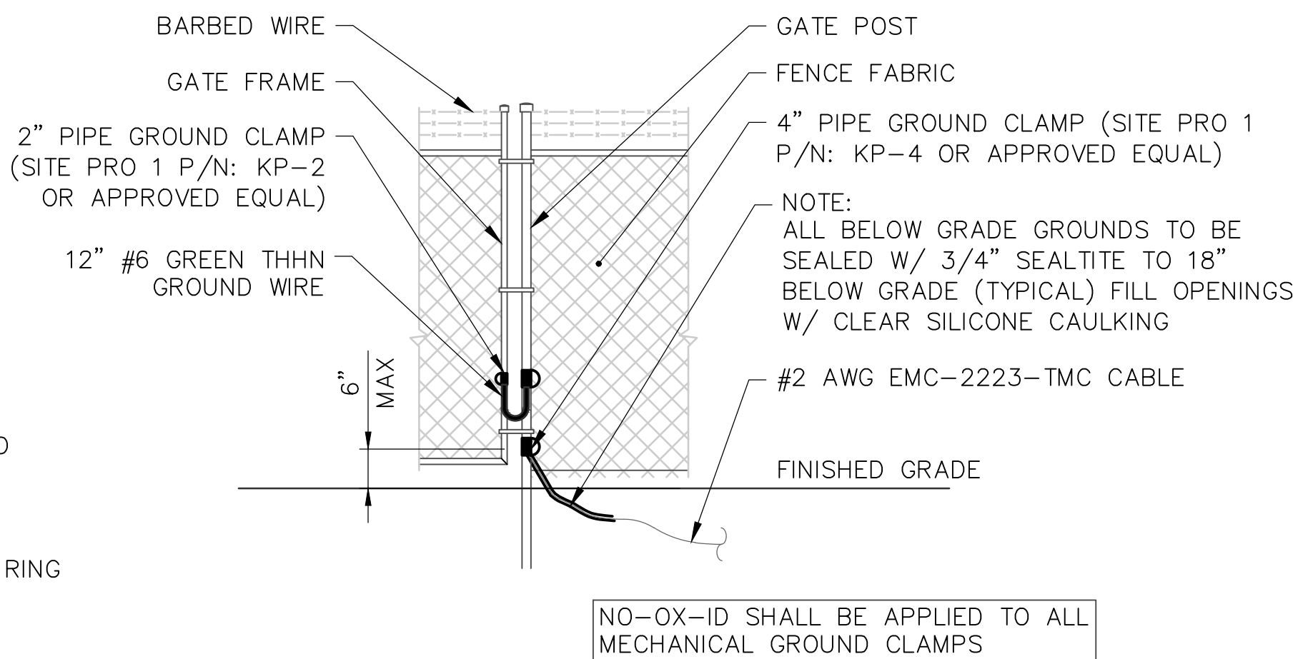
7 GATE GROUNDING DETAIL E-4 SCALE: NTS
