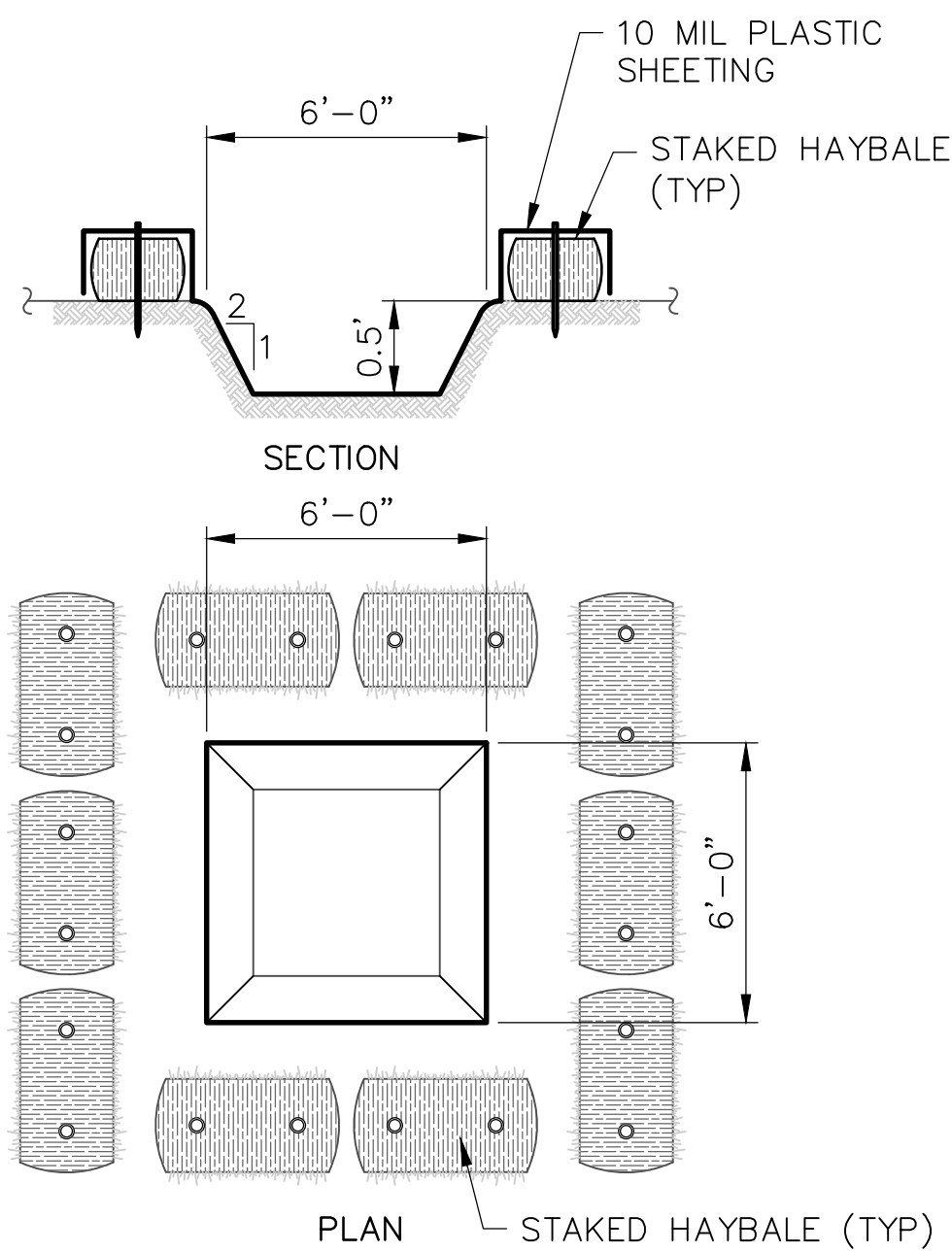
5 TEMPORARY CONCRETE WASH SCALE: NTS
