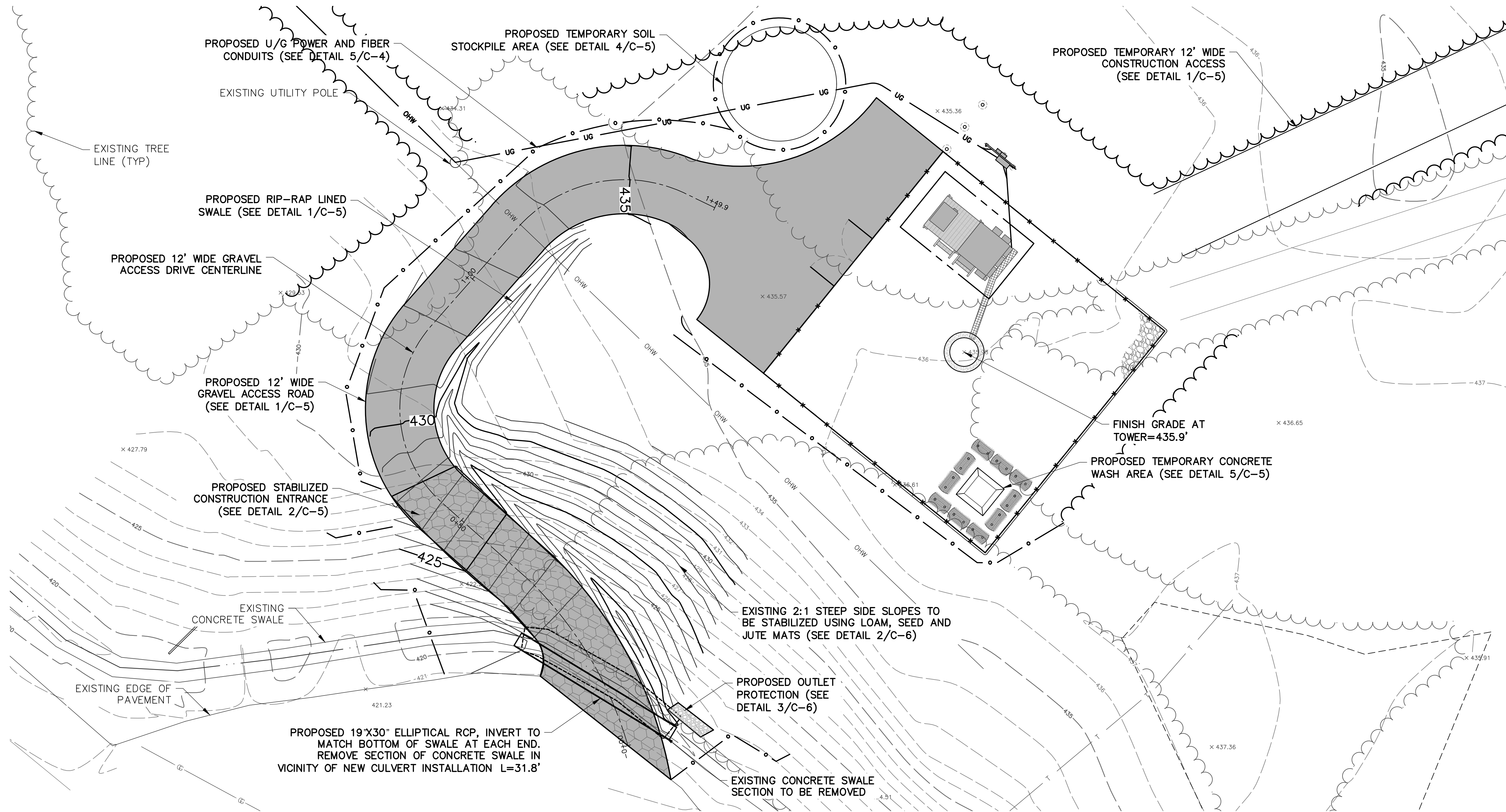
1 C-1B DRIVEWAY PLAN VIEW SCALE: 1" = 20' (11x17 SIZE) 1" = 10' (22x34 SIZE)
