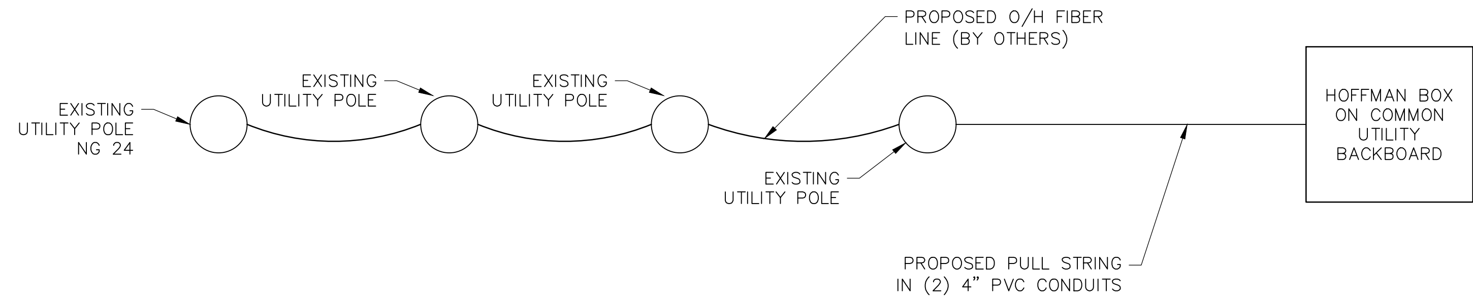
2 TELEPHONE LINE DIAGRAM E-1 SCALE: NTS
