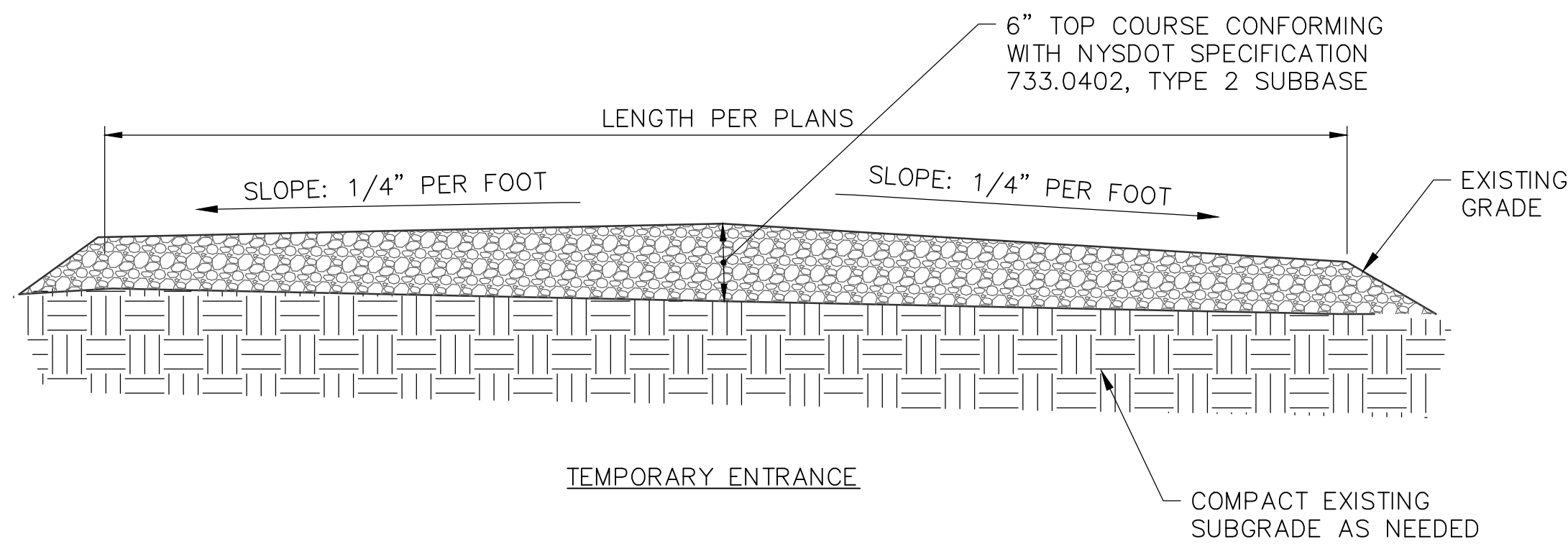
1 GRAVEL DRIVE CROSS SECTIONS SCALE: NTS
