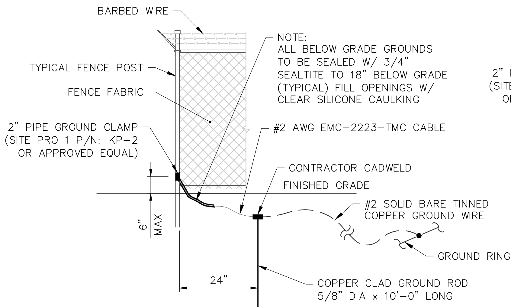
6 FENCE CORNER GROUNDING DETAIL E-4 SCALE: NTS
