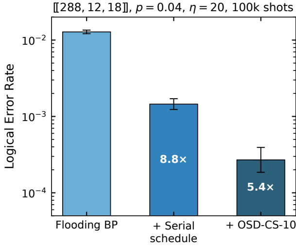
Figure 4: Baseline decomposition on [[288, 12, 18]] , p = 0.04 , \eta = 20 , 100k identical shots. The figure is intended to isolate the effect of serial scheduling. Min-sum BP (scaling 0.8, at most 100 iterations) with flooding and subsequent OSD-CS-10 then serial schedule, then serial BP-OSD-CS-10. Wilson 95% CI error bars; labels give the exact flooding-BP comparator configuration must be reported in the text before the multiplicative factors are interpreted causally factor gained at each step.
