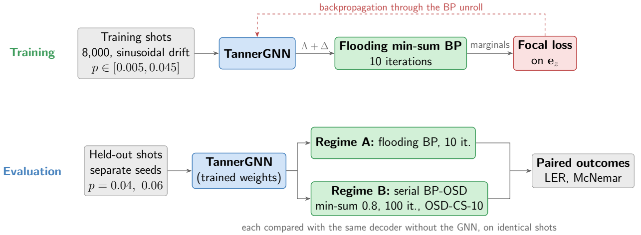
Figure 3: Experimental Training and evaluation pipeline of the GNN experiments . Syndromes are sampled under static or drift noise models The GNN is trained through 10-iteration flooding BP and evaluated on separately seeded held-out shots in Regime A (flooding BP) and Regime B (serial BP-OSD); each decoder receives identical syndrome batches to enable McNemar paired testing. Oracle experiments substitute true per-qubit rates for the uniform mean prior.
