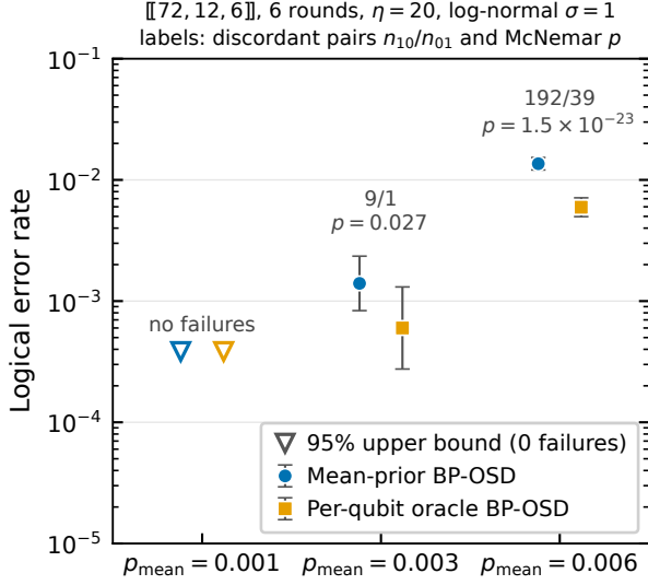
Figure 8: Circuit-level oracle gap on [[72, 12, 6]] , 6 rounds, \eta = 20 , \sigma = 1 . Points: LER with 95% Wilson intervals; open triangles: 95% upper bound when no failures were observed. Labels: discordant pairs and McNemar p .
