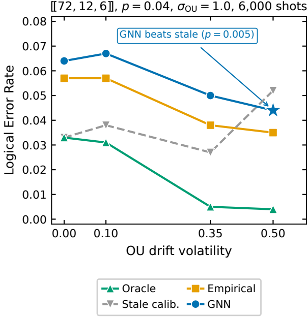
Figure 7: LER vs. OU drift volatility for four decoder configurations on \llbracket 72, 12, 6 \rrbracket , p = 0.04 , \sigma_{OU} = 1.0 , 6,000 shots. Star marks the single operating point (vol=0.5) where GNN beats stale calibration ( p = 0.005 ); GNN is beaten by the empirical frequency estimator at every volatility level.
