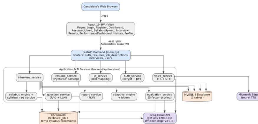
Figure 2.1 — Layered System Architecture and Context of SmartInterview
