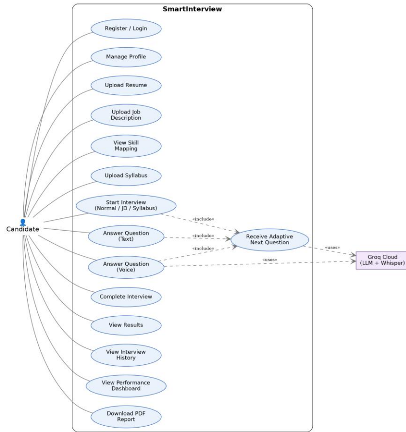
Figure 4.1 — Use Case Diagram for SmartInterview Platform
