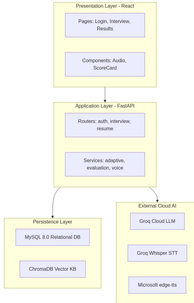
Figure 4.7 — Package Diagram: Layered Subsystem Architecture
