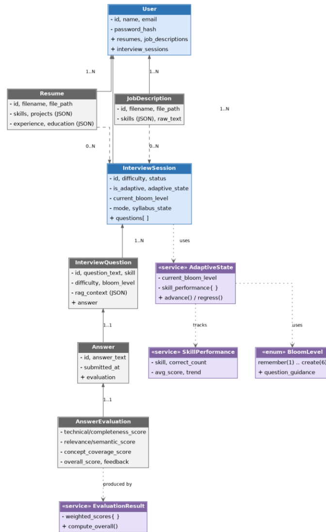
Figure 4.4 — Class Diagram: Relational Model Entities and Service Interfaces
