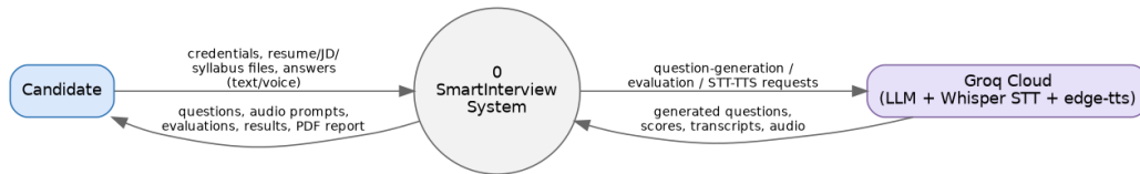
Figure 4.11a — Context-Level Data Flow Diagram (Level 0)
