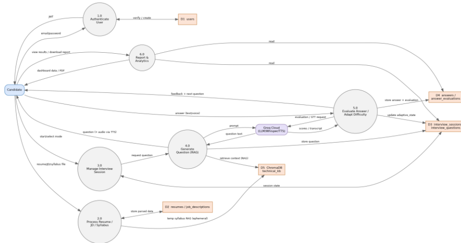
Figure 4.11b — Decomposed Data Flow Diagram (Level 1)
