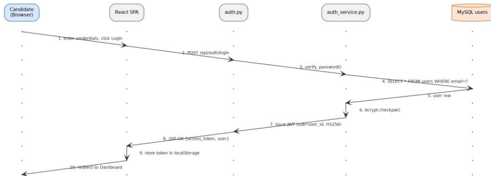
Figure 4.2a — Sequence Diagram: Candidate Authentication and Token Issuance
