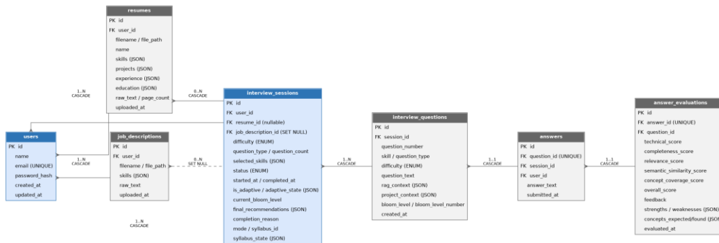
Figure 4.10 — Entity-Relationship Diagram (MySQL 8.0, 7 Relational Tables)
