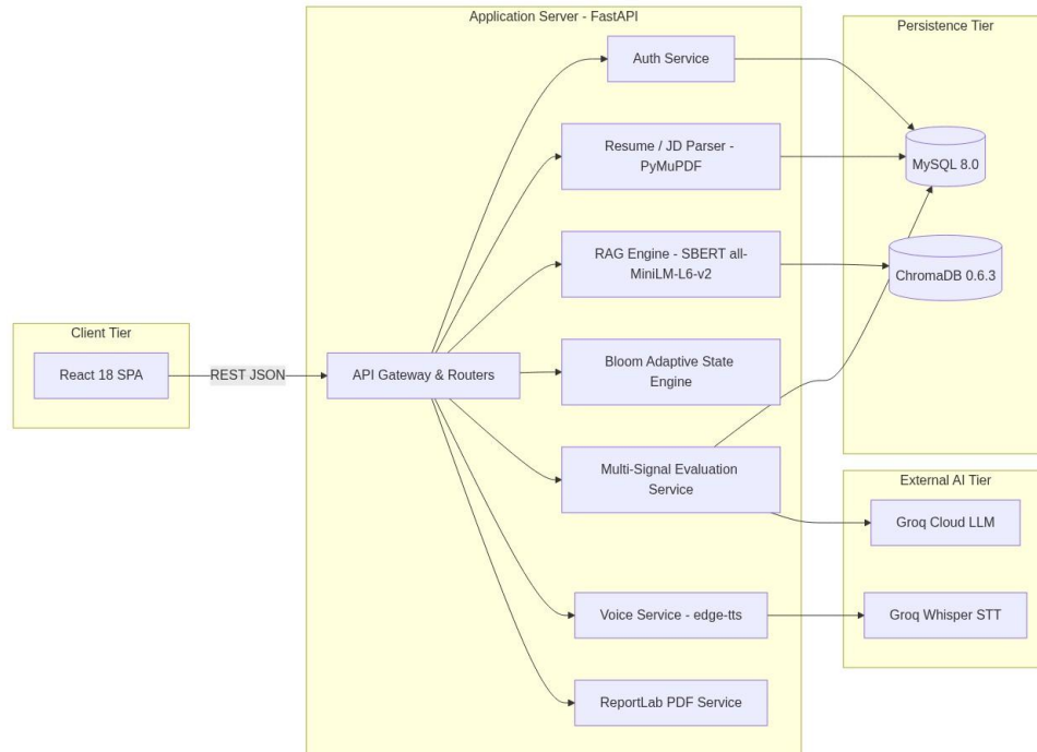
Figure 4.8 — Component Diagram: Internal Service Wiring and External Interfaces
