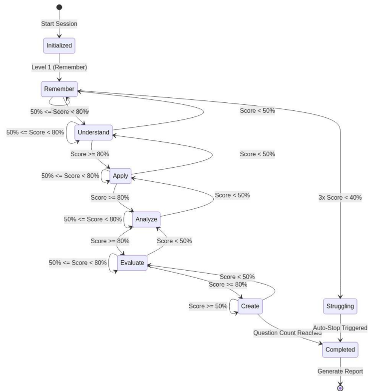
Figure 4.5 — Statechart Diagram: Bloom's Taxonomy Cognitive State Transitions
