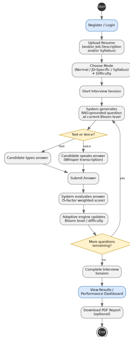
Figure 4.6 — Activity Diagram: End-to-End Candidate Interview Lifecycle
