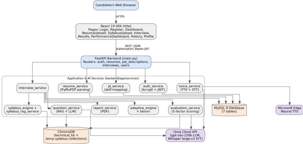
Fig. 1. End-to-end layered system architecture of the SmartInterview platform.
