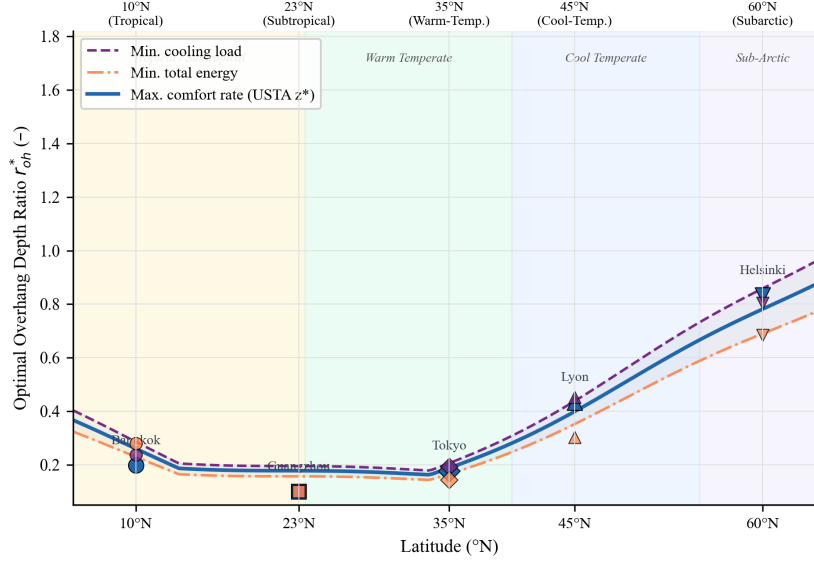
Figure 7: Cross-latitude generalisation: optimal south-facing overhang ratio r_{oh}^* vs. latitude for cooling-proxy minimization (USTA-Full). The transition from cooling-dominated to heating-dominated design strategies is evident at approximately 35°–45°N.
