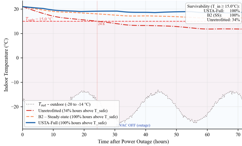
Figure 5: CS2 passive survivability: indoor temperature during 72-hour outage scenario at mid-winter. USTA (3R2C) vs. B2 (steady-state R-value) vs. unretrofitted baseline.
