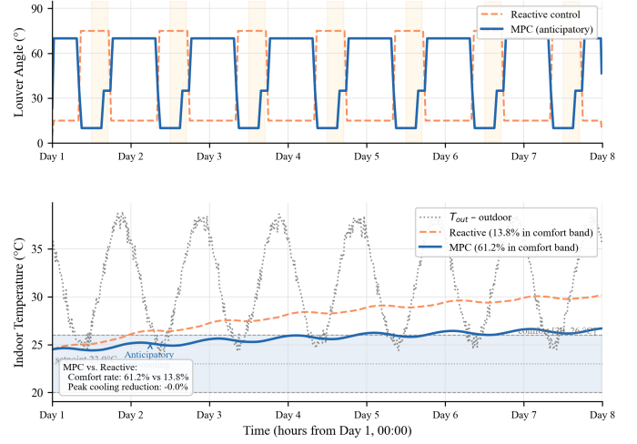
Figure 6: CS3 MPC performance over a representative 7-day period. Upper: lower angle ( \theta_{low} ) trajectory for USTA-Full (MPC) vs. B3 (reactive). Lower: indoor temperature T_{in} with comfort band [T_{low}, T_{high}] . MPC pre-closes louvers before occupancy surge at 14:00.
