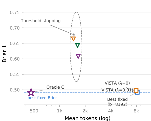
(a) Quality-Compute Frontier (M1 / MMLU-Pro)
