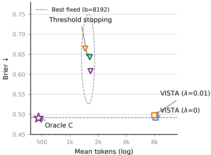
(a) Quality-Compute Frontier (M1 / MMLU-Pro)
