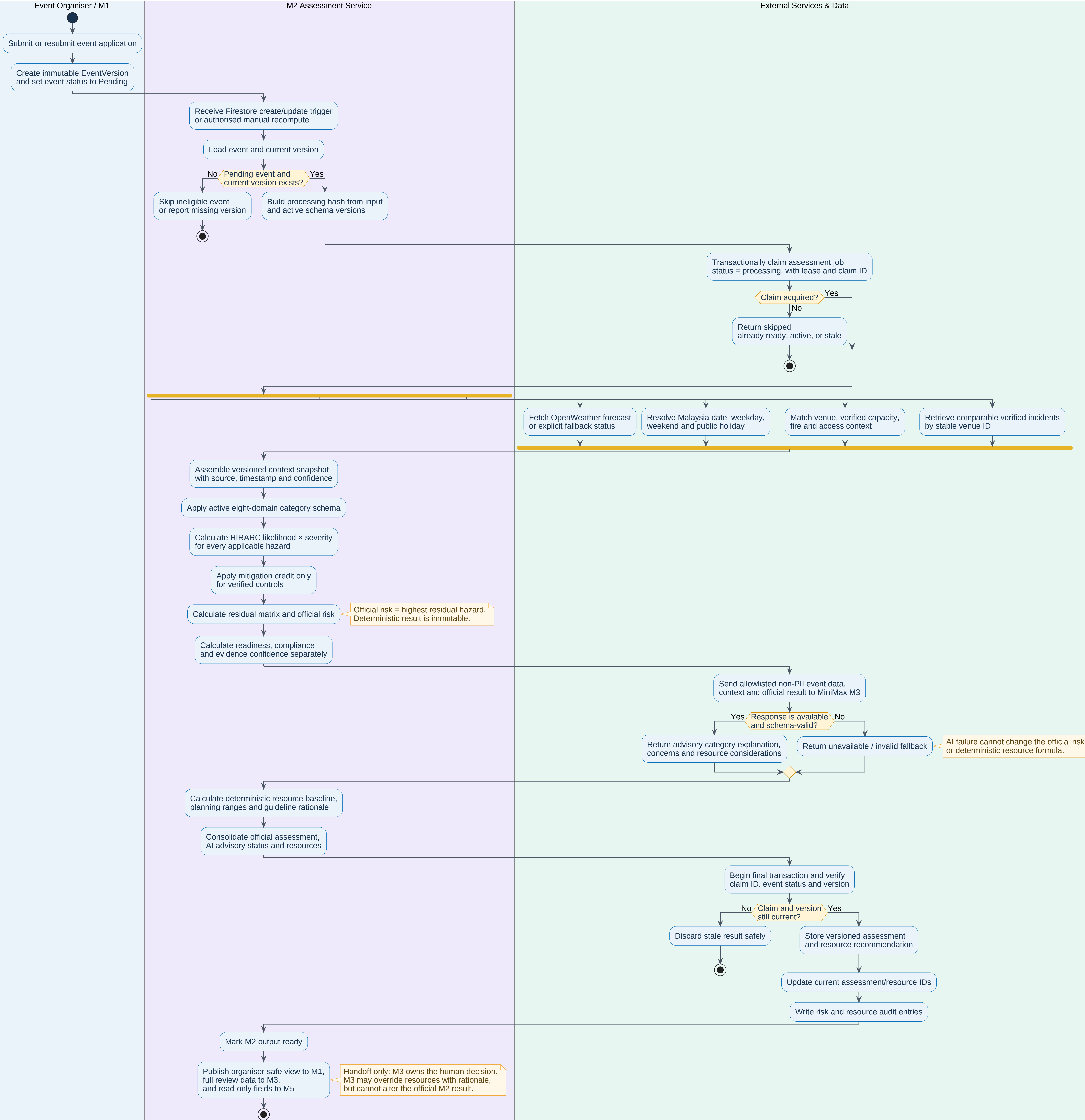
M2 — Smart Risk Assessment and Safety Resource Recommendation Activity Diagram
