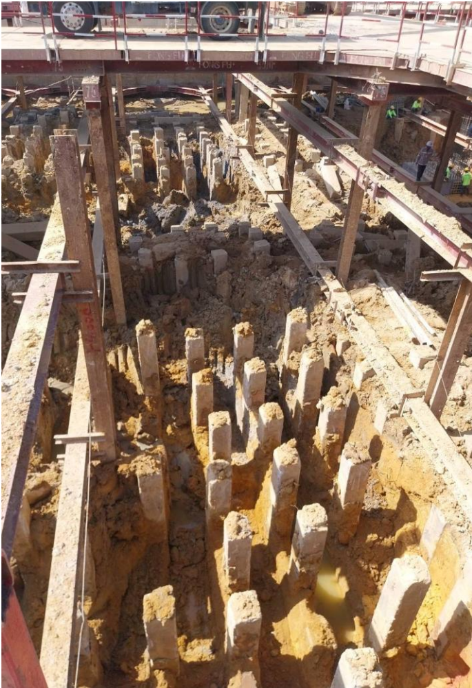
Cutting Piles
