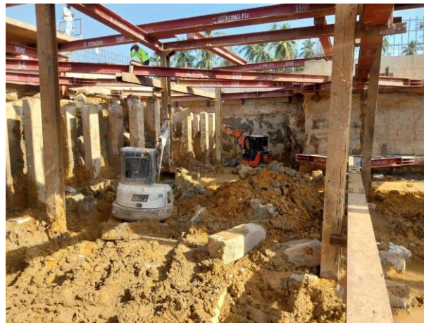
Excavations work
