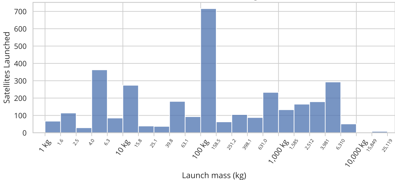
Satellite Launch Mass (excluding Starlink)
