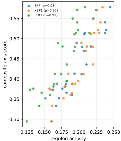
Highest- \rho regulators vs axis (naive B, per-donor)
