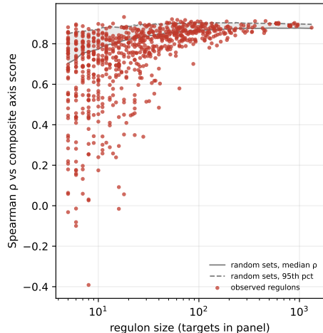
Regulon activity vs axis score (B naive) target-number-matched random-set envelope
