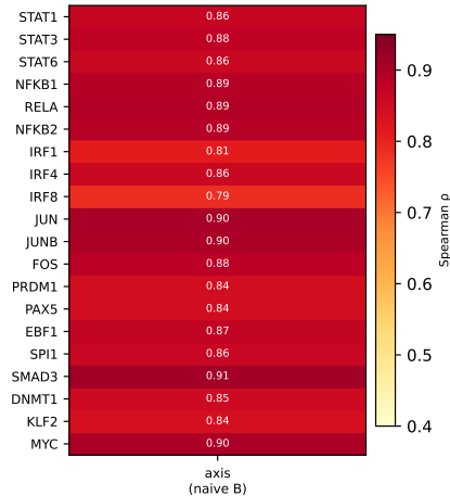
Pre-specified candidate TFs (cytokine / B-cell / epigenetic machinery)
