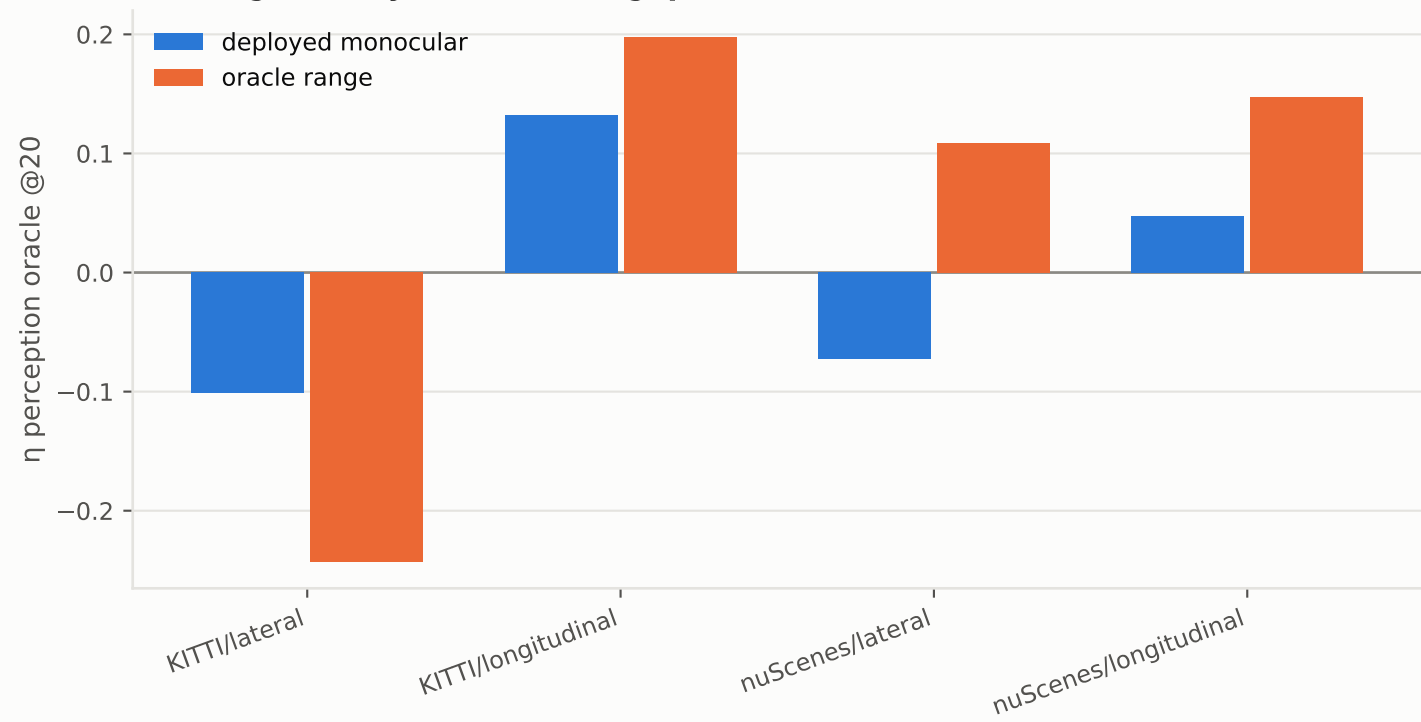
Better geometry narrows the gap but does not close it
