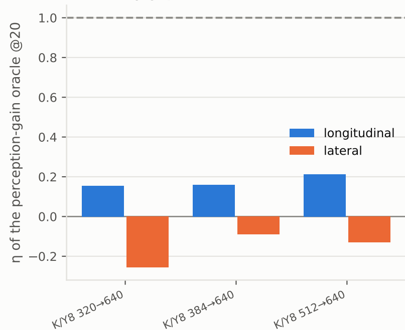
07 fidelity gap (KITTI/YOLOv8s)
