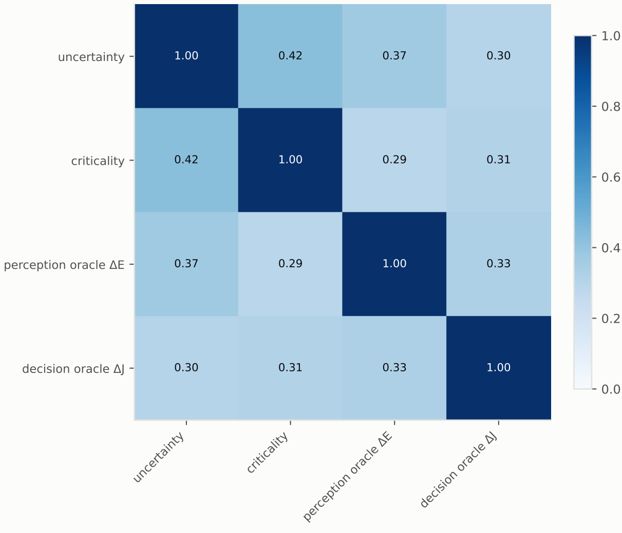
overlap of the top 20% frames — plannerC_path_dev
