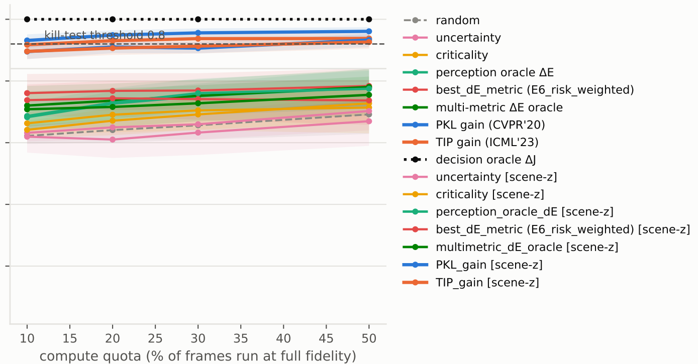
Planner C (PKL's own planner), path deviation
