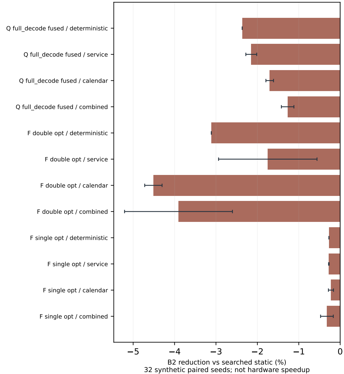
Aggregate attention / resident conditioning
