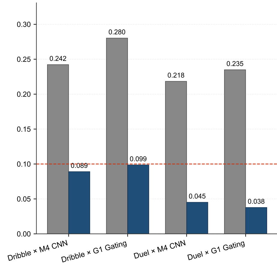
ECE (lower = better)
