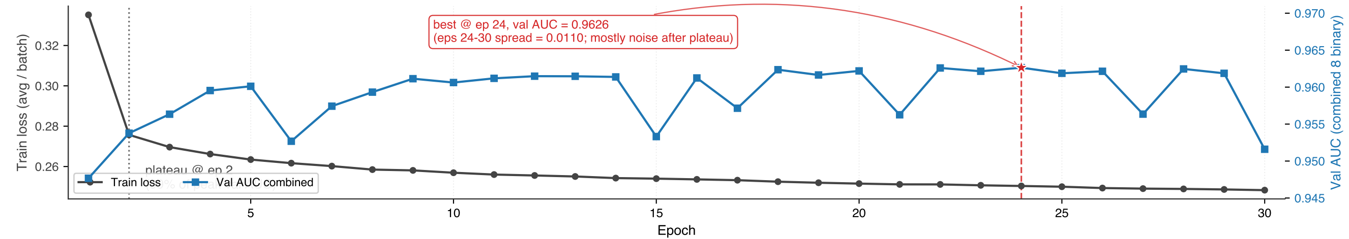
(a) Train loss & combined val AUC vs epoch (raw, no smoothing)
