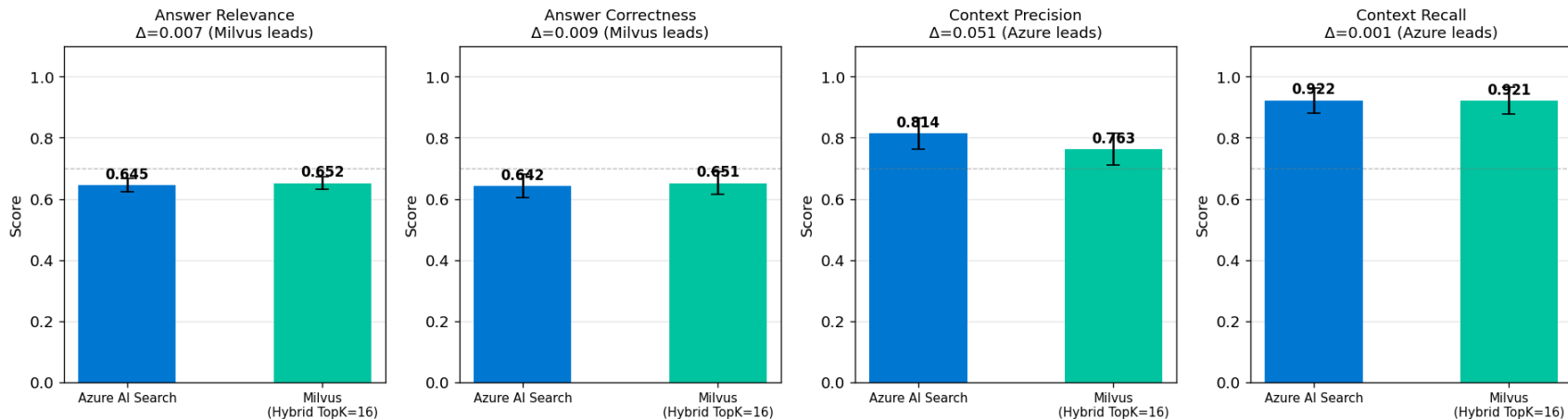
Mean Score per Metric — Azure AI Search vs Milvus Hybrid (TopK=16) error bars = 95% CI
