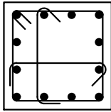
TYPE E 12 BARS (4 × 4) TIE + 2 CROSSTIES
