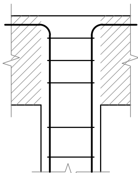
(a) INTERIOR: HOOKS OUTWARD
