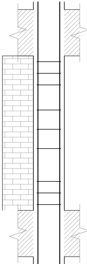
(b) FULL INFILL ON ONE SIDE l o ZONES @ s 0 ; MID ZONE ≤ 2 s 0 AND ≤ d/2
