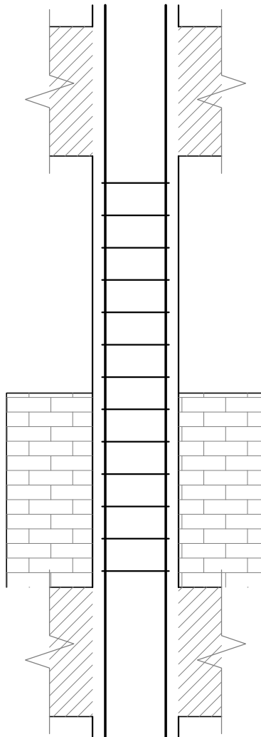
(a) PARTIAL-HEIGHT INFILL HOOPS @ s 0 OVER THE FULL HEIGHT; SHEAR FOR THE SHORT COLUMN; HOOPS ≥ c 1 INTO THE WALL ZONE
