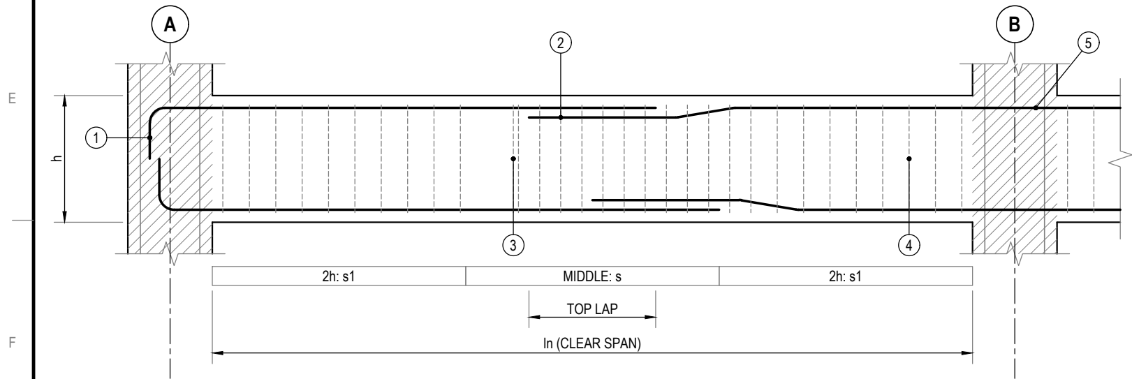
BEAM - SPECIAL MOMENT FRAME
