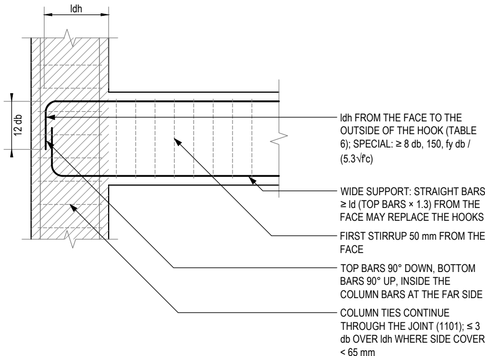
BEAM END AT AN EXTERIOR COLUMN
