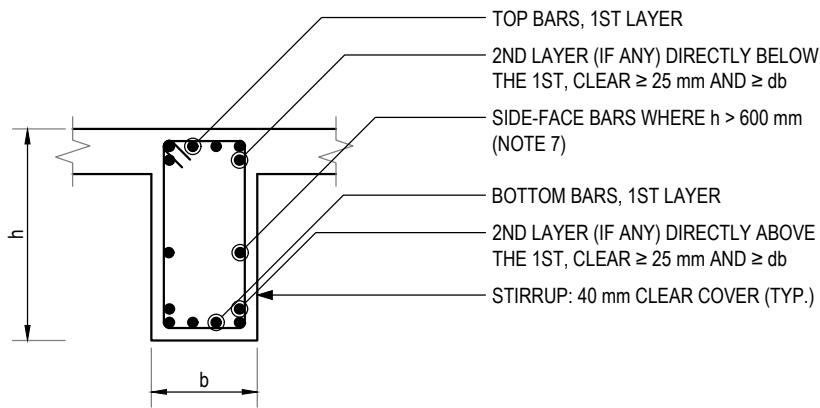
TYPICAL BEAM SECTION
