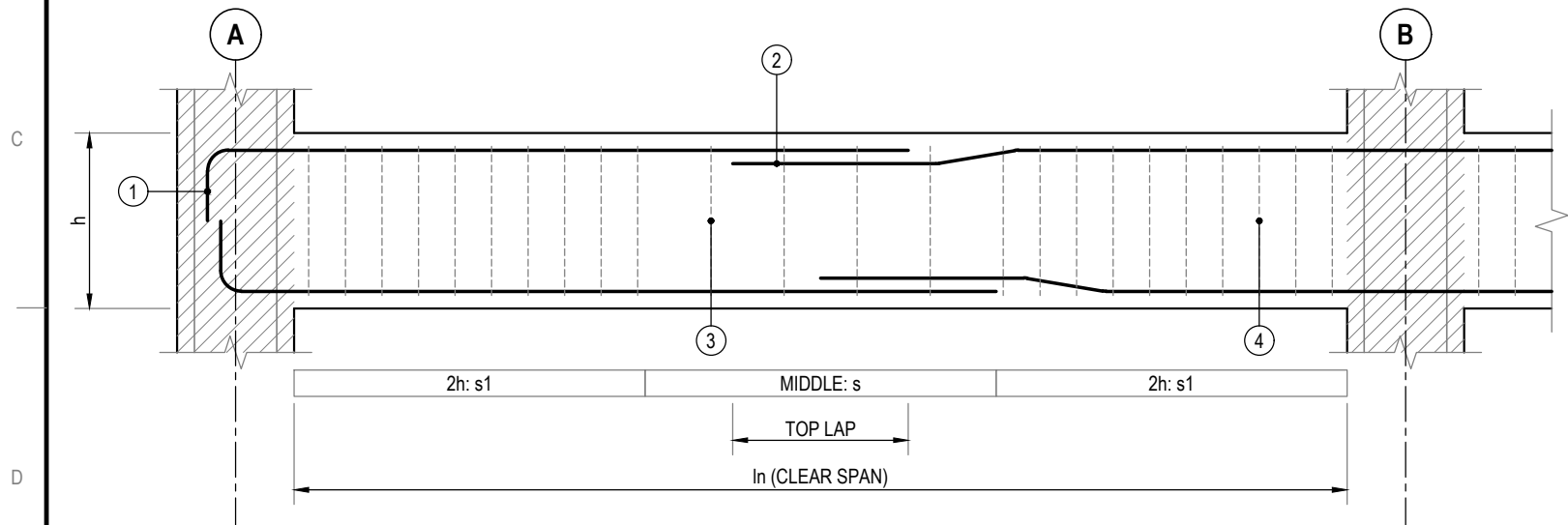
BEAM - INTERMEDIATE MOMENT FRAME
