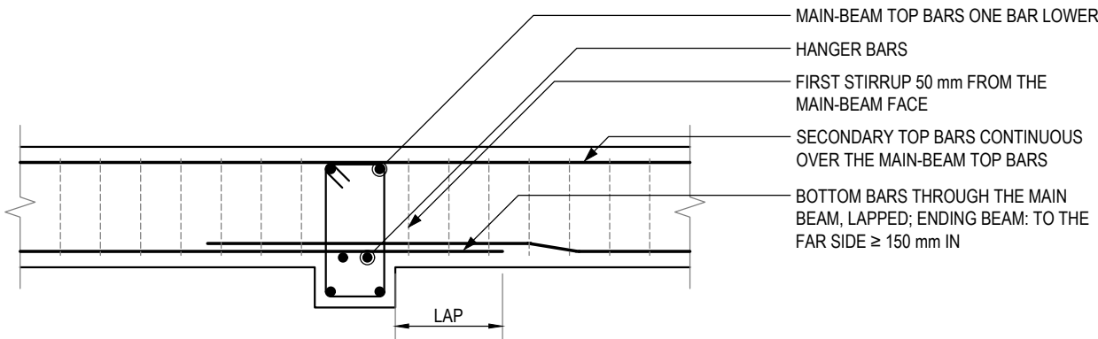
SECTION ALONG THE SECONDARY BEAM
