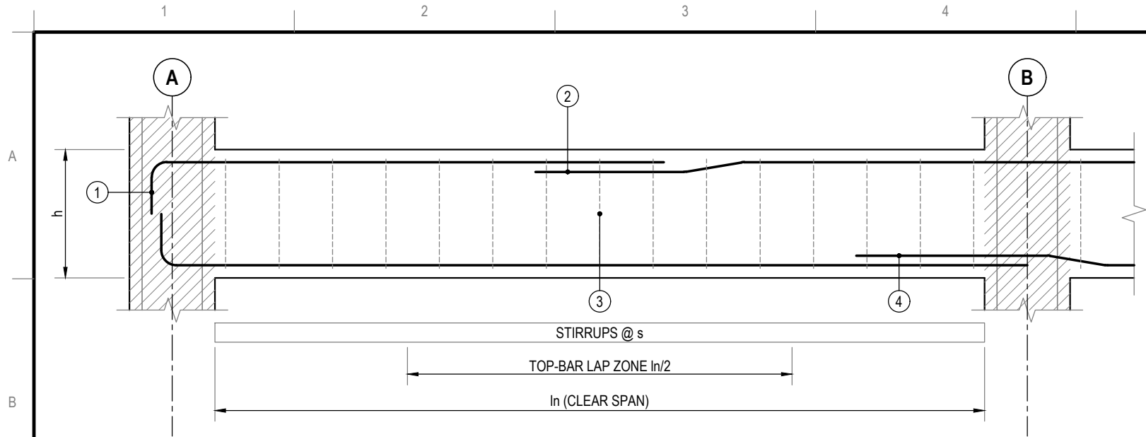
BEAM - ORDINARY MOMENT FRAME
