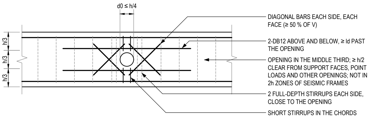
OPENING THROUGH THE WEB
