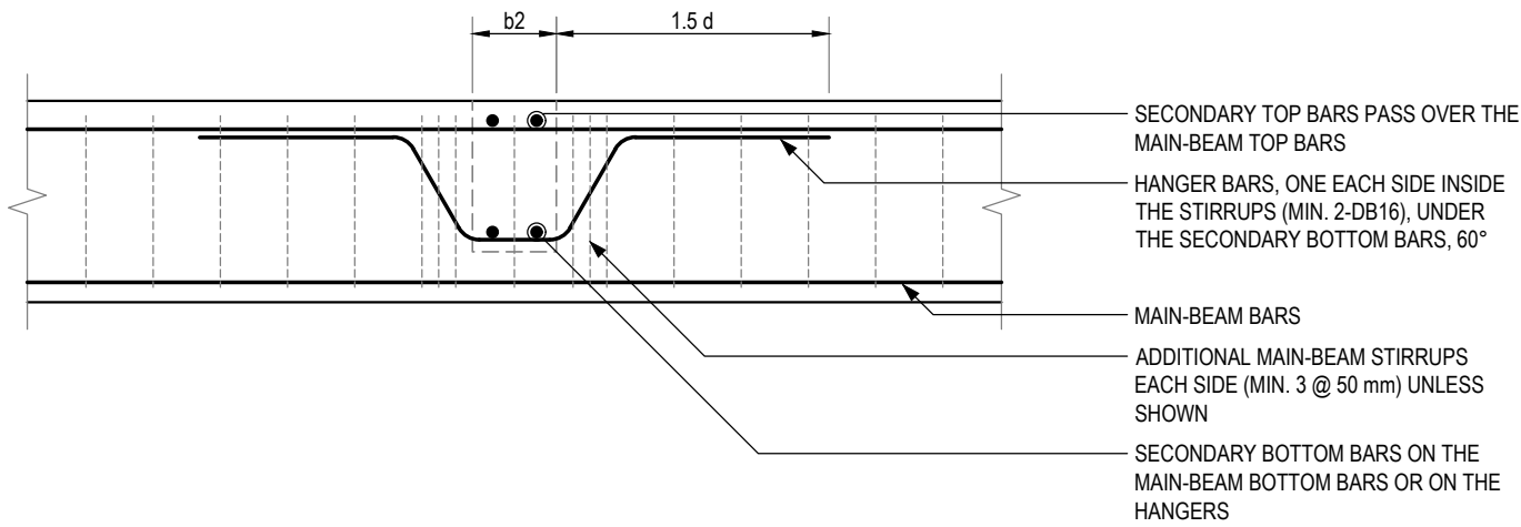
SECONDARY BEAM ON A MAIN BEAM
