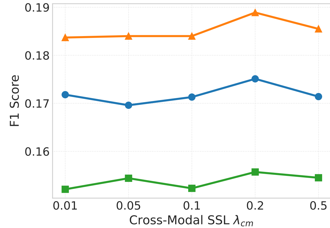
(c) Effect of \lambda_{cm}
