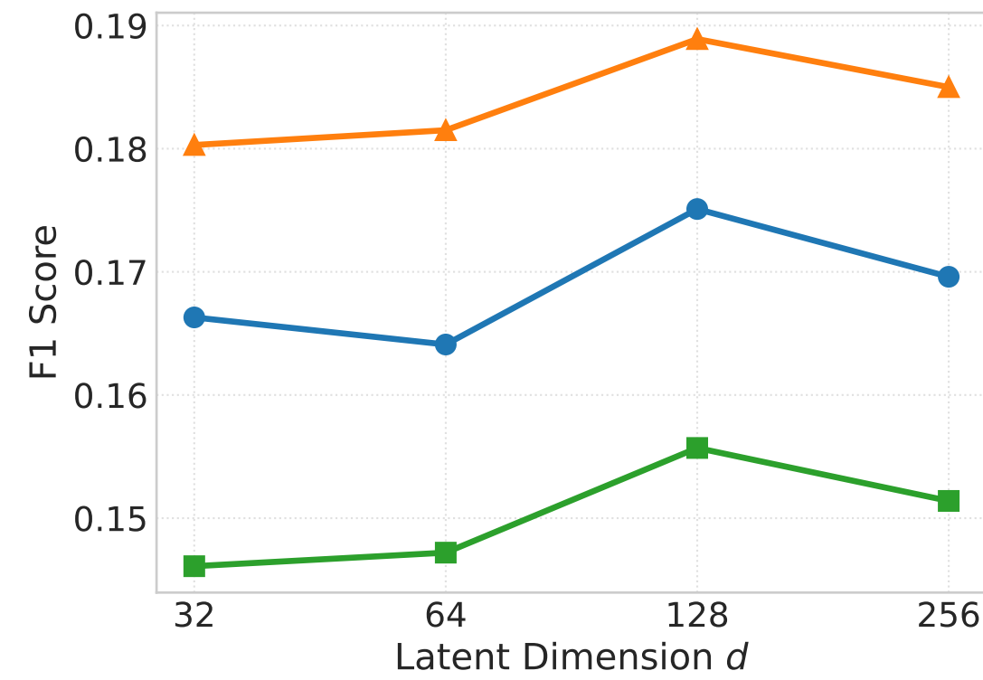
(f) Effect of Dimension d
