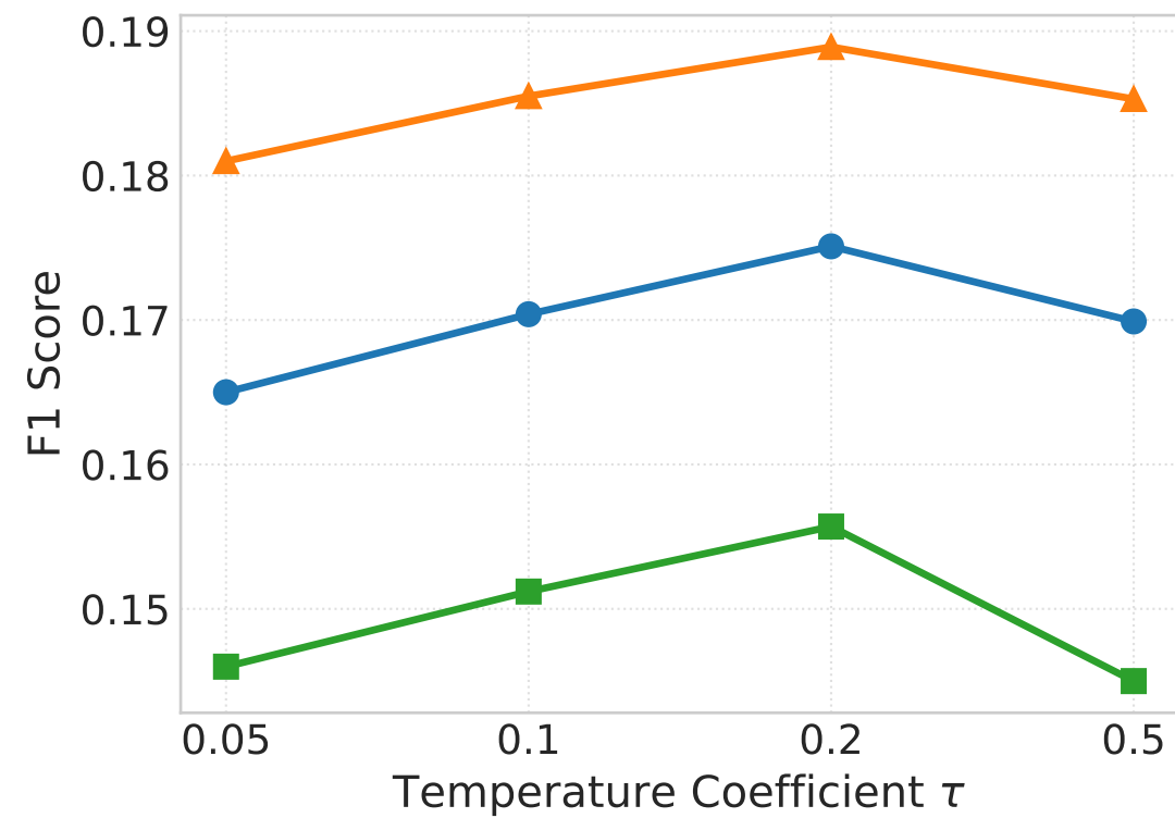
(e) Effect of Temperature \tau
