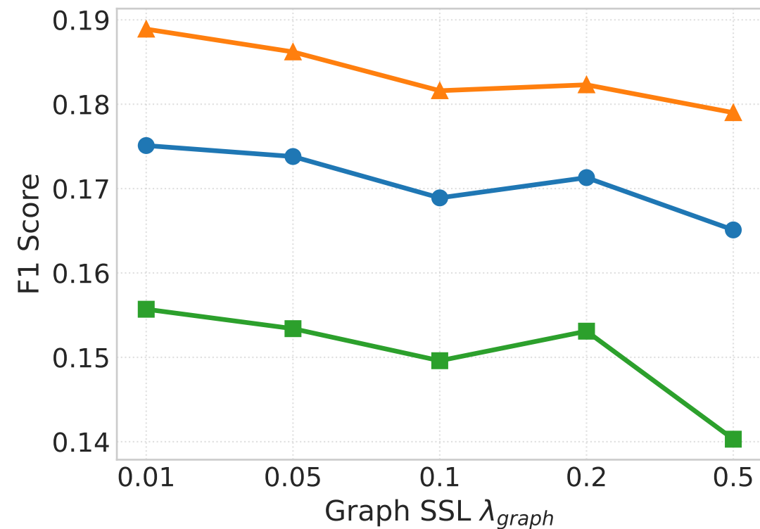
(b) Effect of \lambda_{graph}
