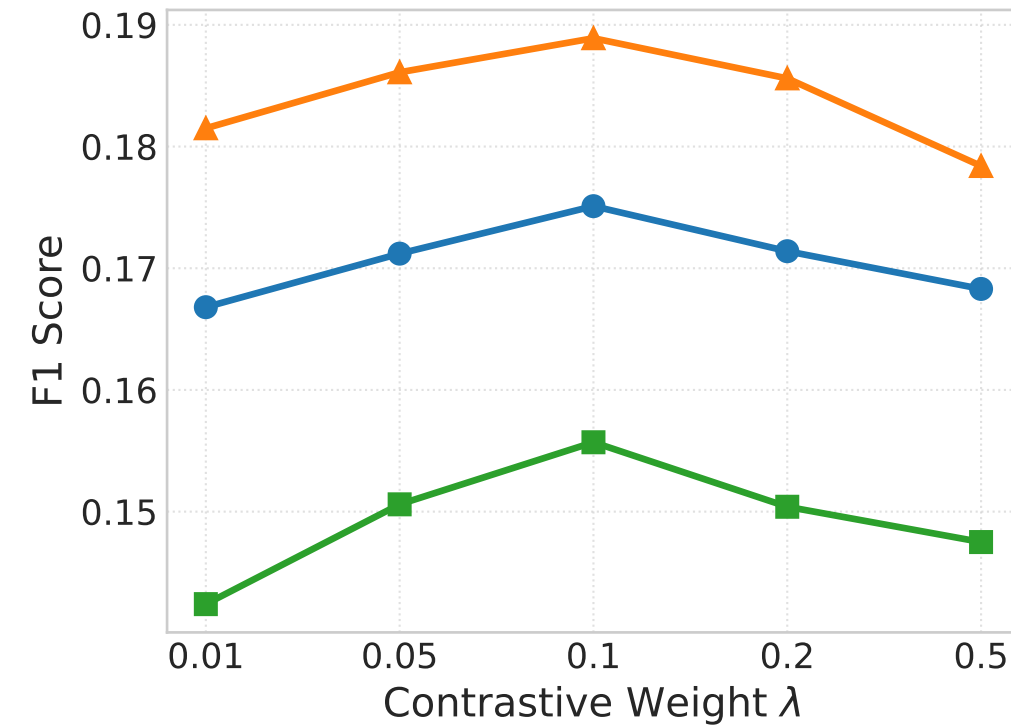
(b) Effect of Weight \lambda
