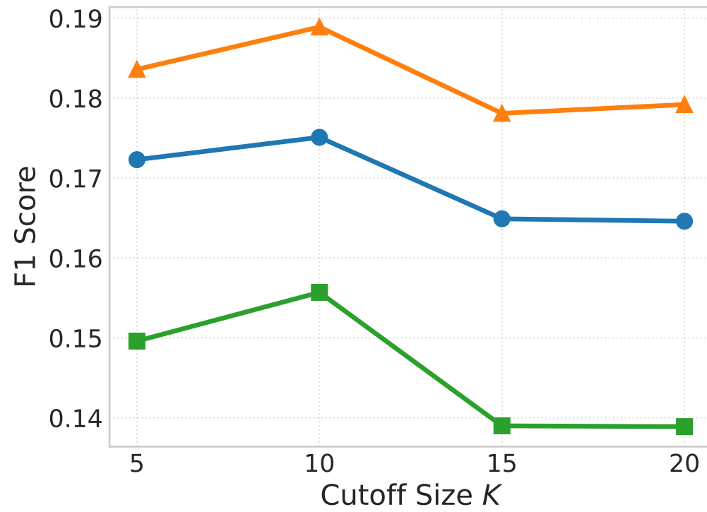
(a) Effect of Cutoff Size K
