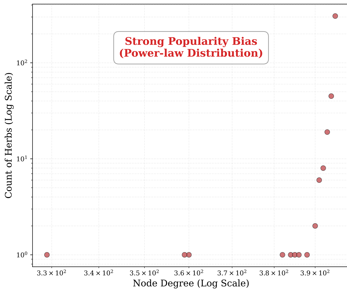
(c) Raw Graph Node Degree Distribution
