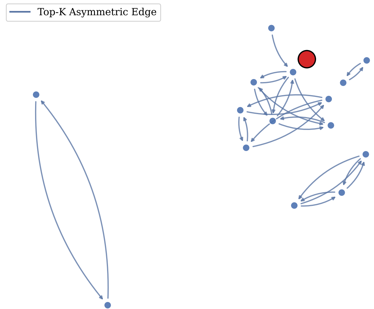
(b) Pruned Asymmetric Collaborative Graph
