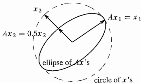
Ax lines up with x at eigenvectors
