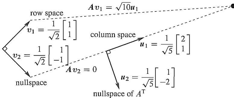
Figure 6.9: The SVD chooses orthonormal bases for 4 subspaces so that A\mathbf{v}_i = \sigma_i \mathbf{u}_i .
