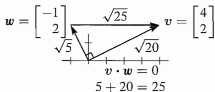
Figure 1.8: Perpendicular vectors have v \cdot w = 0 . Then \|v\|^2 + \|w\|^2 = \|v - w\|^2 .
