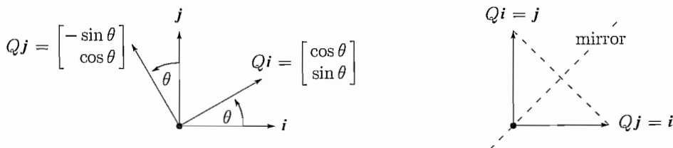
Figure 4.10: Rotation by Q = \begin{bmatrix} \cos \theta & -\sin \theta \\ \sin \theta & \cos \theta \end{bmatrix} and reflection across 45^\circ by Q = \begin{bmatrix} 0 & 1 \\ 1 & 0 \end{bmatrix} .
