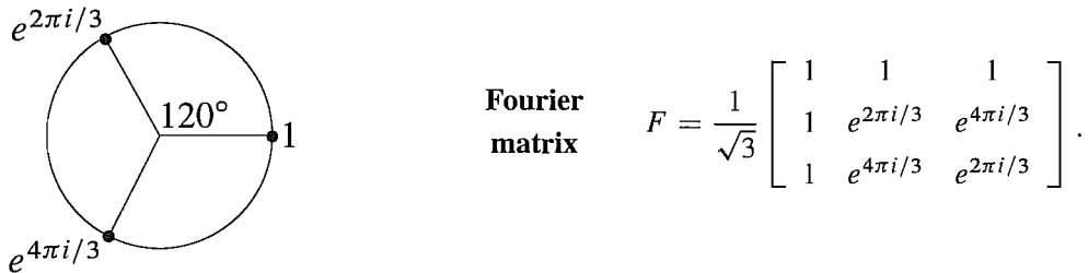
Figure 10.3: The cube roots of 1 go into the Fourier matrix F = F_3 .
