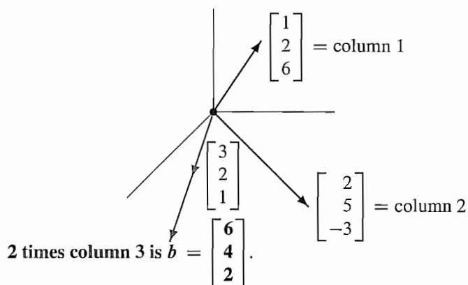
Figure 2.4: Column picture: (x, y, z) = (0, 0, 2) because 2(3, 2, 1) = (6, 4, 2) = \mathbf{b} .
