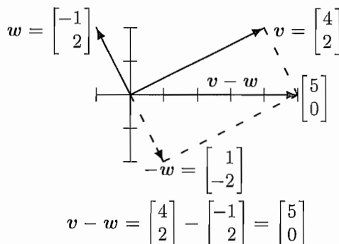
Figure 1.1: Vector addition v + w = (3, 4) produces the diagonal of a parallelogram. The linear combination on the right is v - w = (5, 0) .
