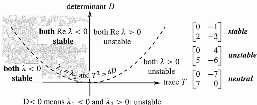
Figure 6.5: A 2 by 2 matrix is stable ( \mathbf{u}(t) \rightarrow \mathbf{0} ) when trace < 0 and det > 0 .
