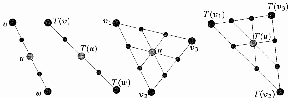
Figure 7.1: Lines to lines, equal spacing to equal spacing, u = \mathbf{0} to T(u) = \mathbf{0} .
