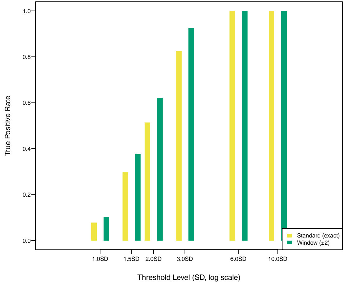
SSVS Performance: Standard vs Window ( \pm 2 ) Window approach allows \pm 2 units tolerance
