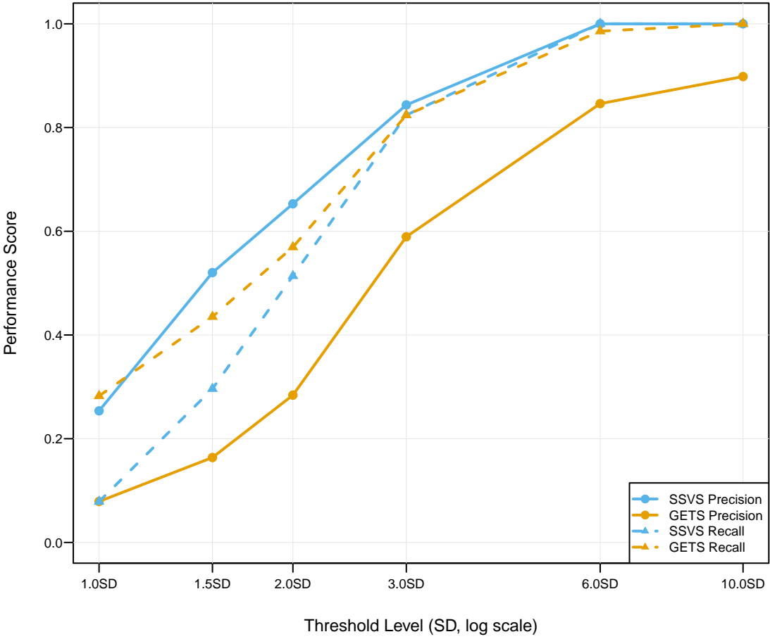
Performance Metrics: SSVS vs GETS Solid lines: Precision, Dashed lines: TP Rate
