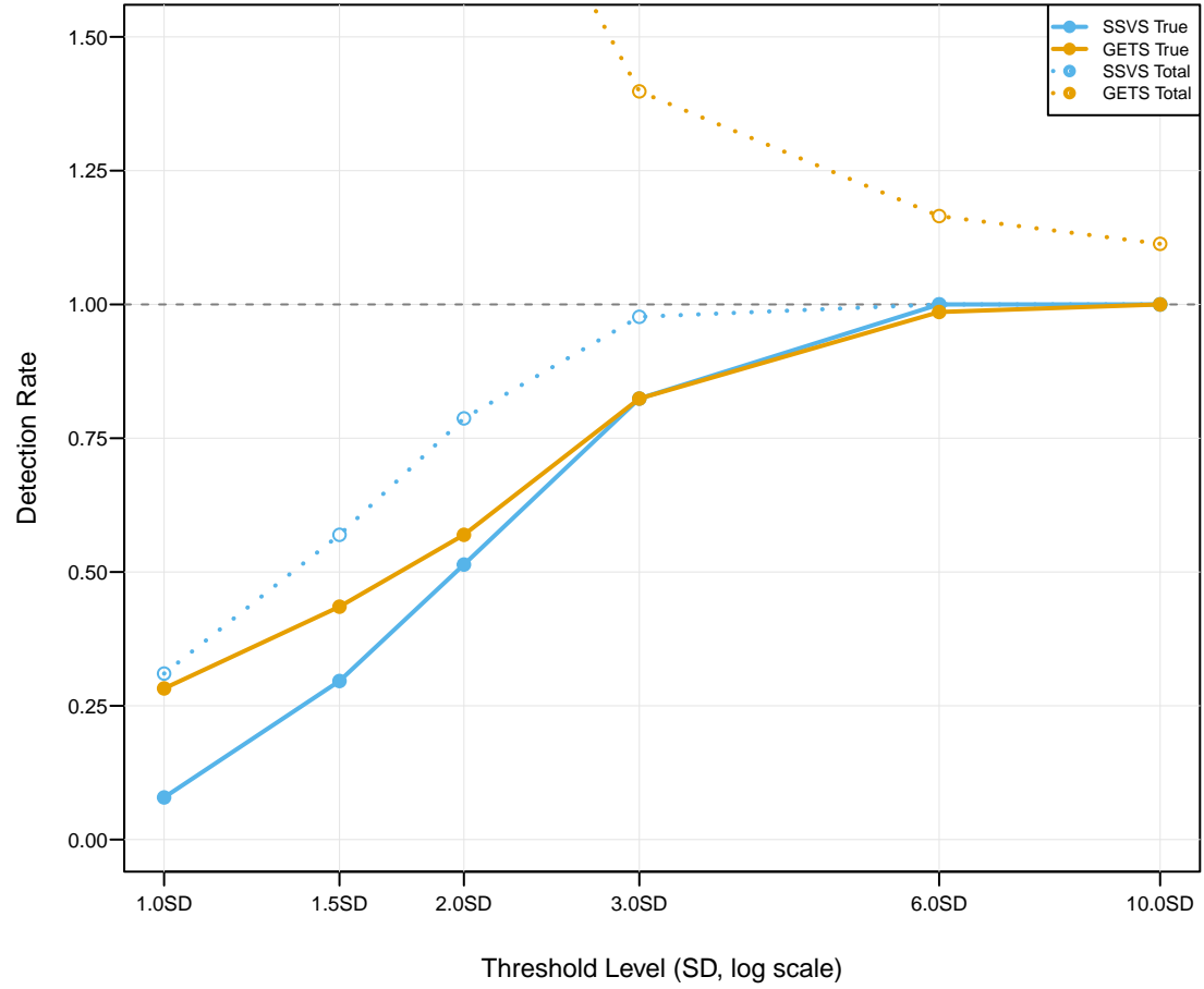
Detection Rates Solid: True detection rate, Dotted: Total detection rate
