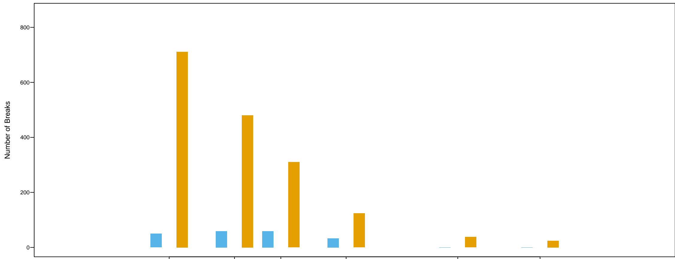
False Positives
