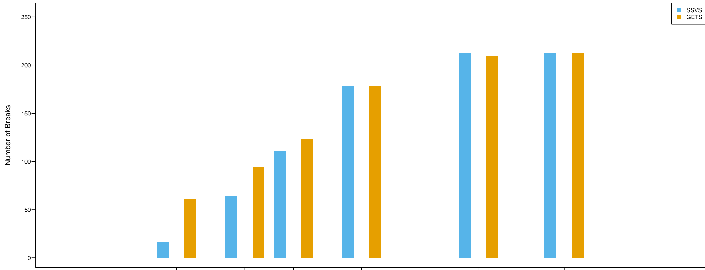
True Positives
