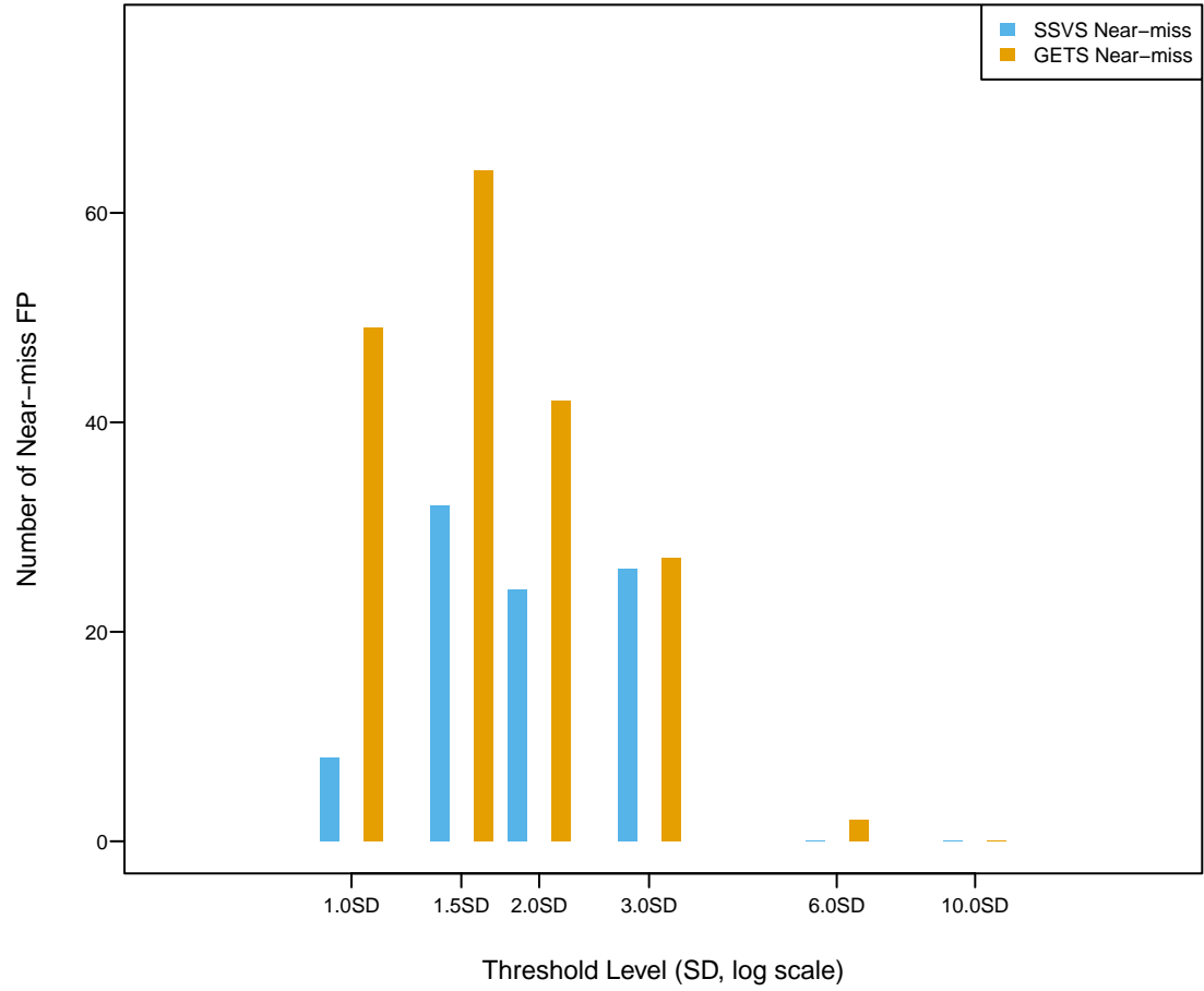
Near-miss False Positives ( \pm 1 unit) False positives within one unit of true break
