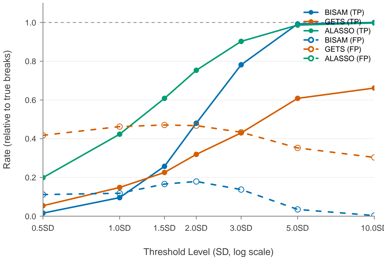
True and False Positive Rates
