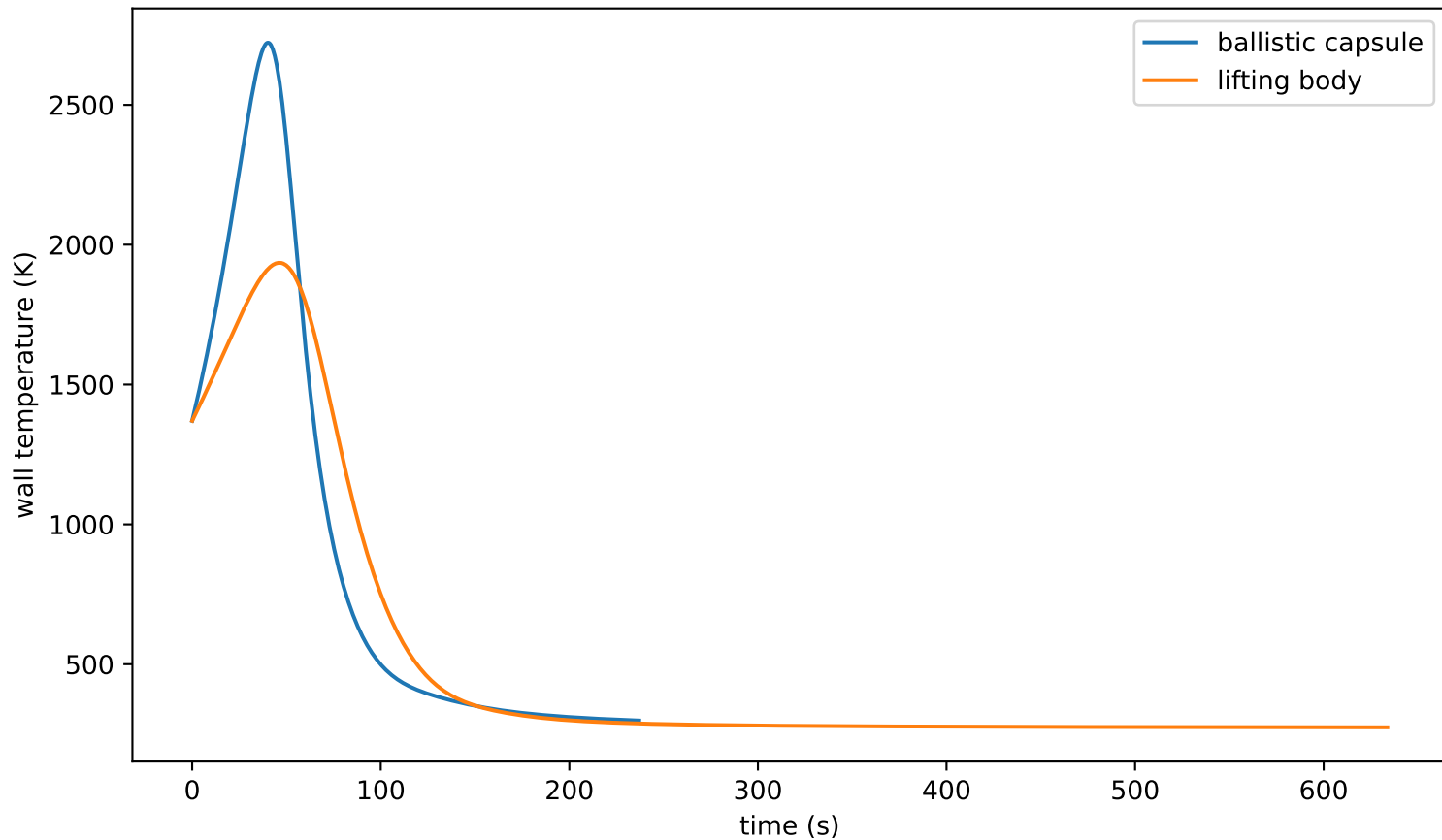
wall temperature comparison
