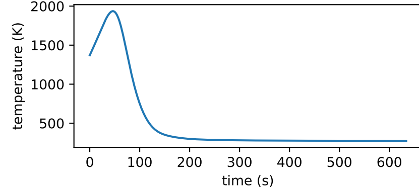
adiabatic wall temperature
