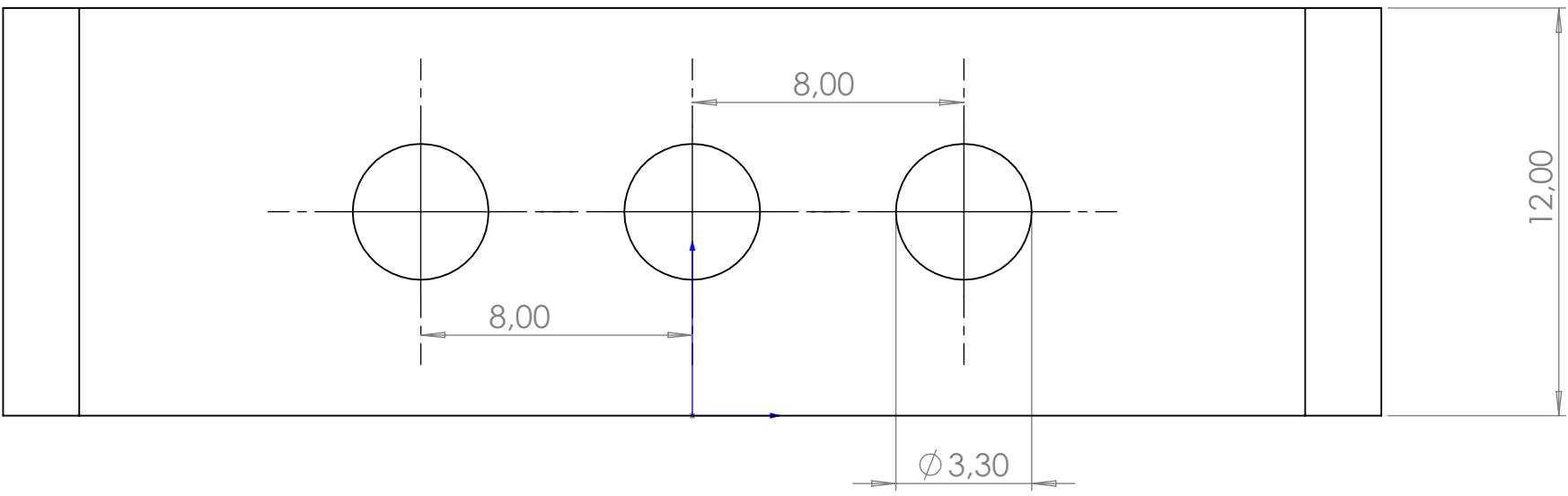
Lateral projection
