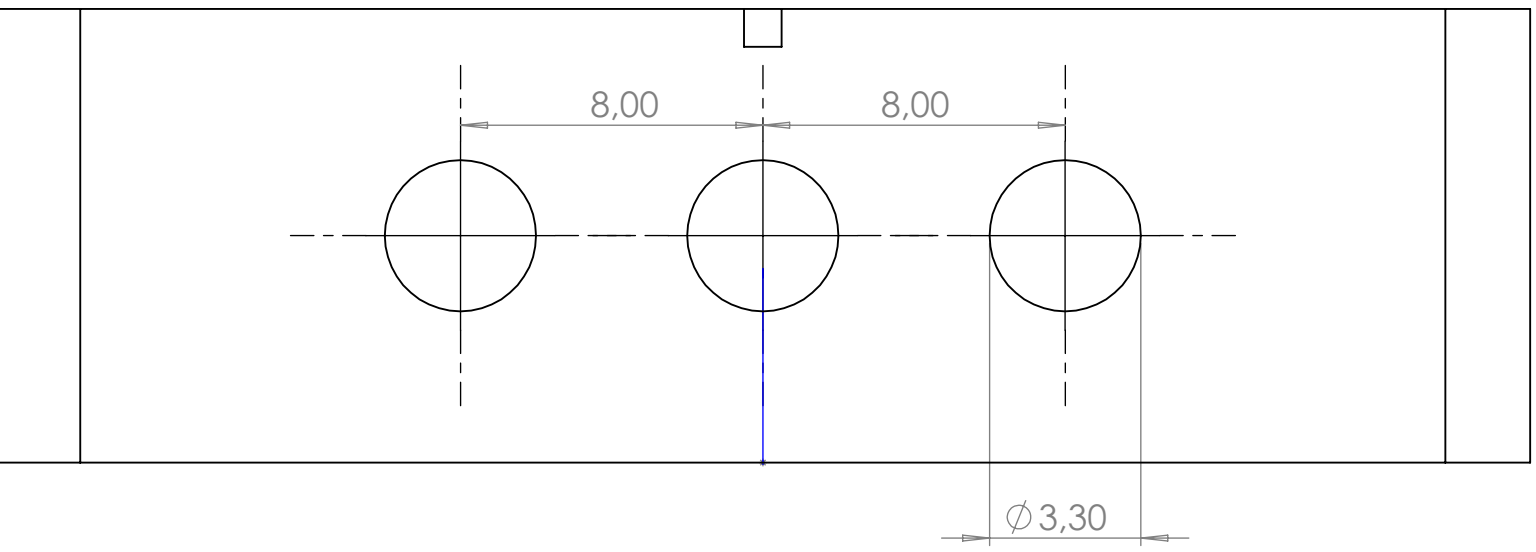
Frontal projection
