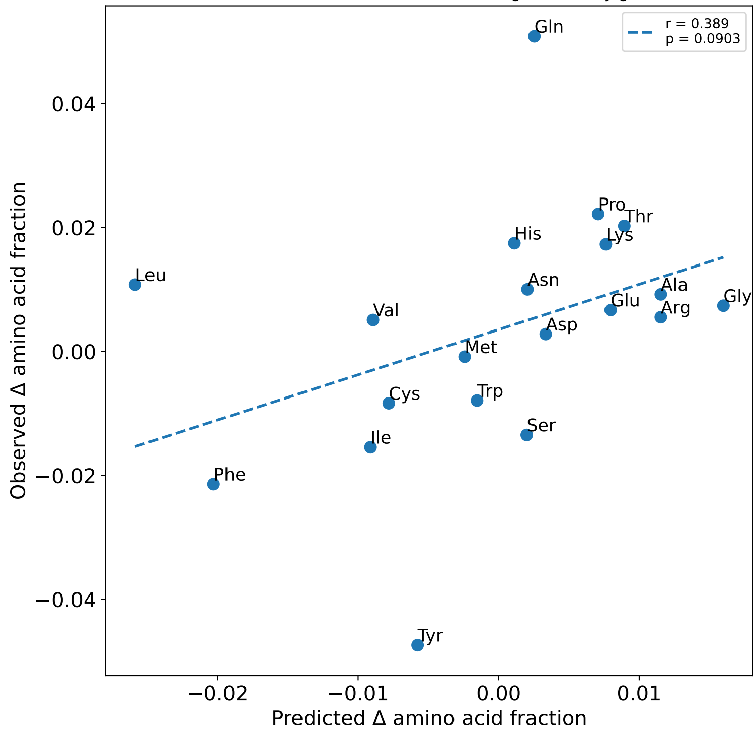
Observed vs Predicted amino acid changes in heavy genes
